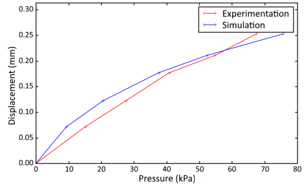
Figure 2 – Experimental and simulated displacements of pressure applied at the top of the bead.
