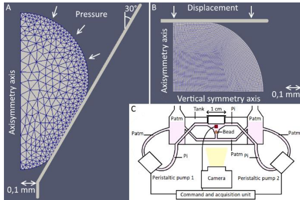
Figure 1 – Finite elements models and their boundary conditions for conical (A) and planar (B) compression – Scheme of the home-made device (C).
