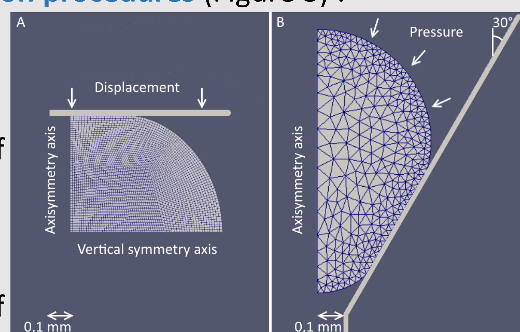
Figure 3 – Finite elements models and their boundary conditions for planar (A) and conical (B) compression – LMGC90.
