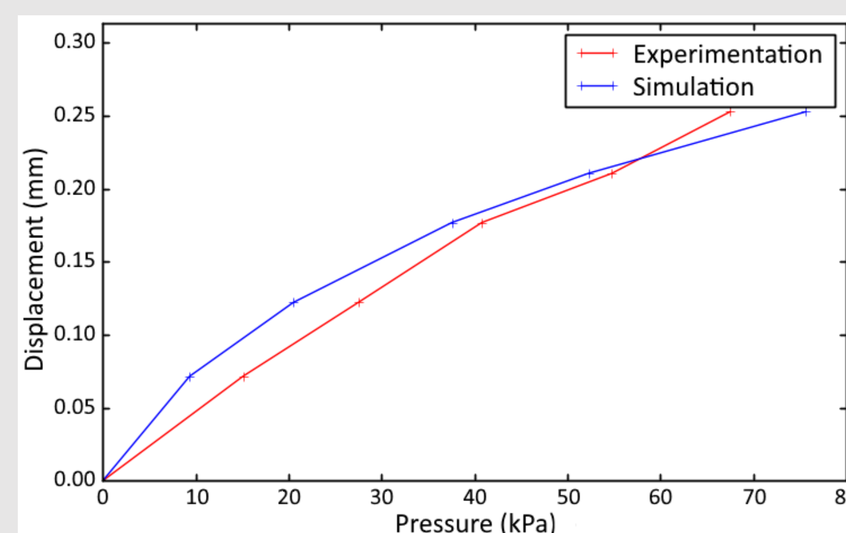
Figure 4 – Experimental and simulated displacements of the bottom of an alginate bead as a function of the pressure applied at the top of the bead.
