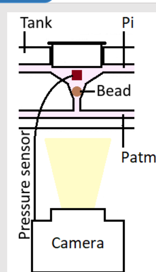
Figure 1 – Fluidic system of compression for microspheres.
