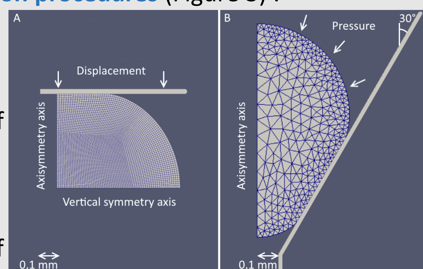
Figure 3 – Finite elements models and their boundary conditions for planar (A) and conical (B) compression – LMG90.
