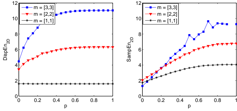
Figure 7: DispEn 2D (left panel) and SampEn 2D (right panel) calculated from MIX 2D processes of size 256 × 256 pixels. The parameters were set to \mathbf{m} = \{[1, 1], [2, 2], [3, 3]\} for both the methods, c = 5 for DispEn 2D and r = 0.24 of image standard deviation for SampEn 2D .
