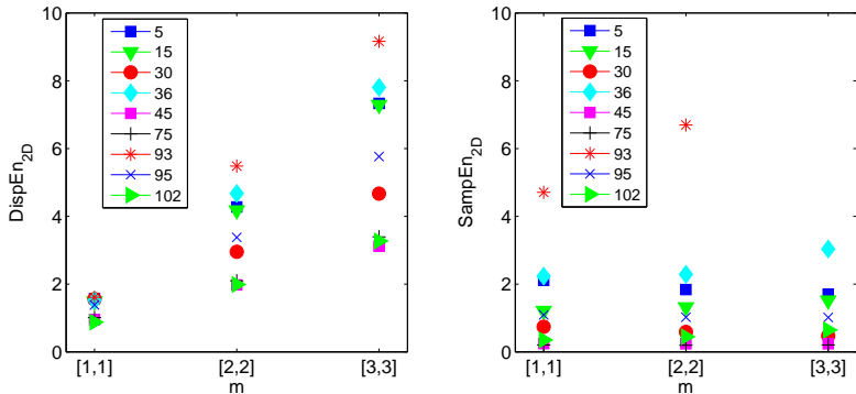
Figure 8: \text{DispEn}_{2D} (left panel) and \text{SampEn}_{2D} (right panel) calculated from the Brodatz dataset presented in Figure 5. The parameters were set to \mathbf{m} = \{[1, 1], [2, 2], [3, 3]\} for both methods, c = 5 for \text{DispEn}_{2D} and r = 0.24 of image standard deviation for \text{SampEn}_{2D} . For \text{SampEn}_{2D} and data 93 at \mathbf{m} = [3, 3] the computation leads to infinite value.
