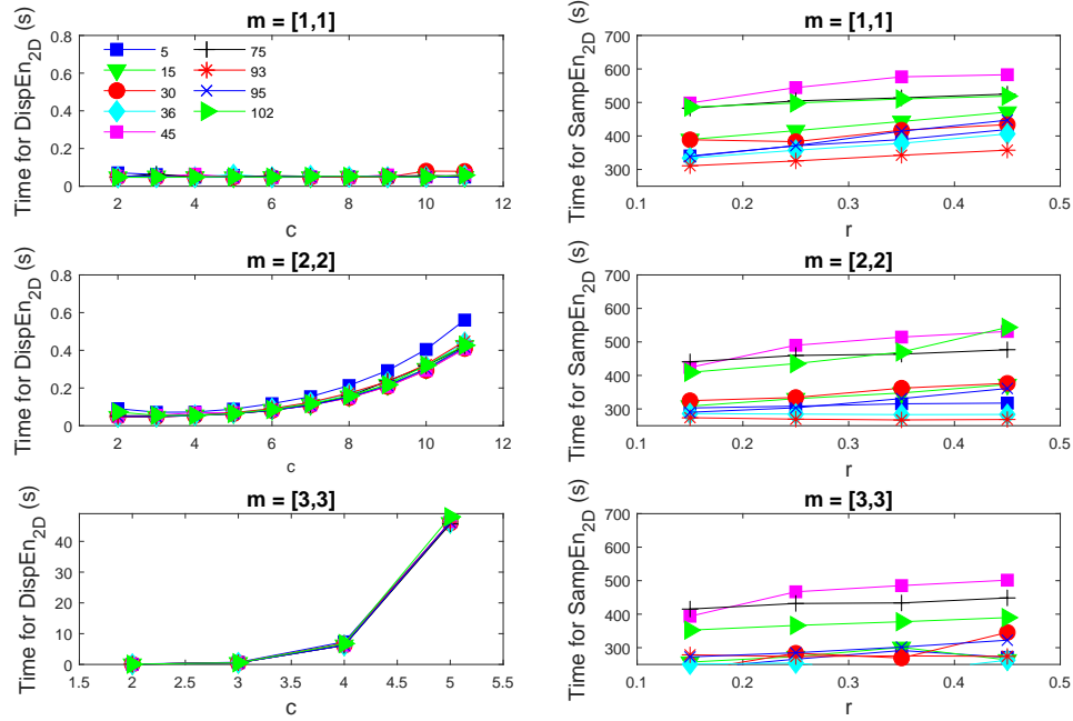
Figure 11: Computational time for \text{DispEn}_{2D} (left panels) and \text{SampEn}_{2D} (right panels) calculated using the Brodatz dataset (images sized 128 \times 128 pixels), for different values of parameters \mathbf{m} , c and r .
