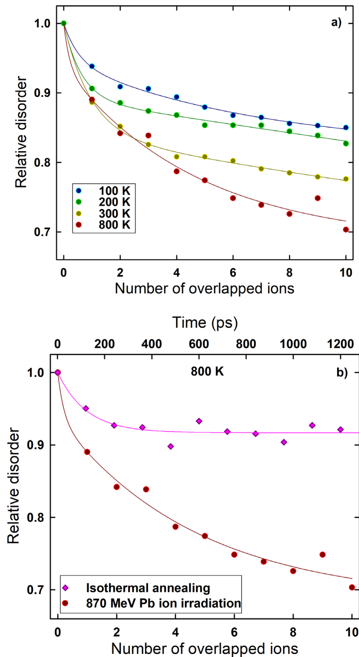
Figure 2: Variation of the MD-derived relative disorder in SiC as a function of a) the number of overlapped SHIs and for different temperatures (see labels), and b) the number of overlapped SHIs and the time for both SHIs and thermal annealing. Lines are fits to experimental data using a double exponential decay function.
