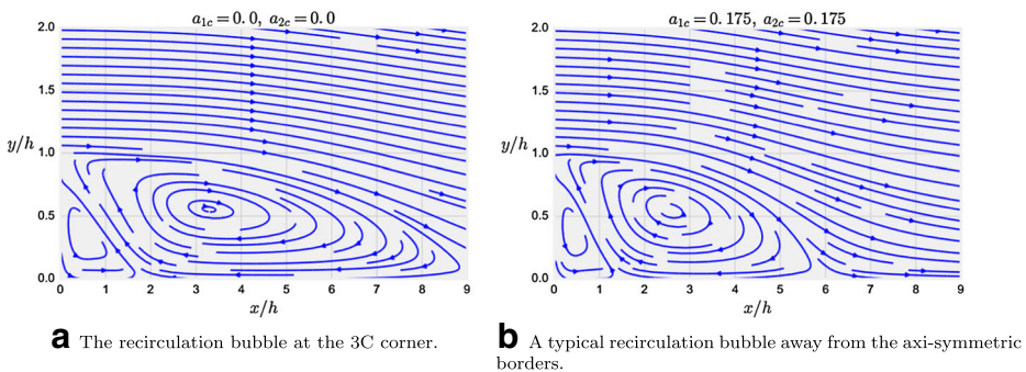
Fig. 16 Two distinctly different recirculation bubbles
