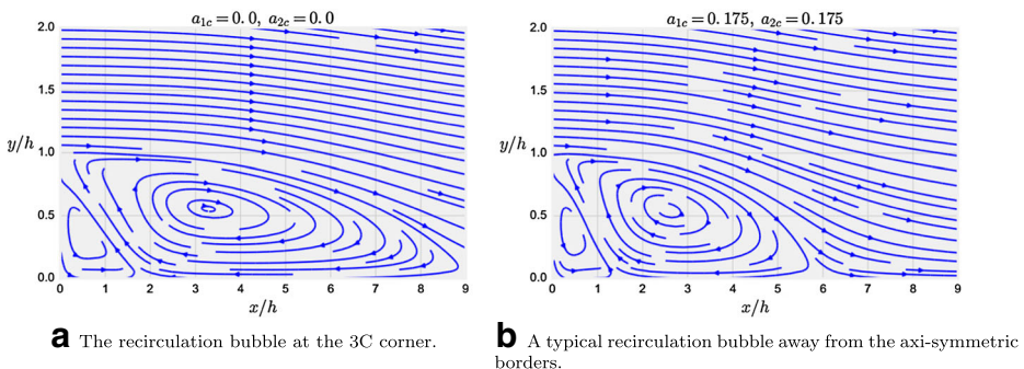
Fig. 16 Two distinctly different recirculation bubbles
