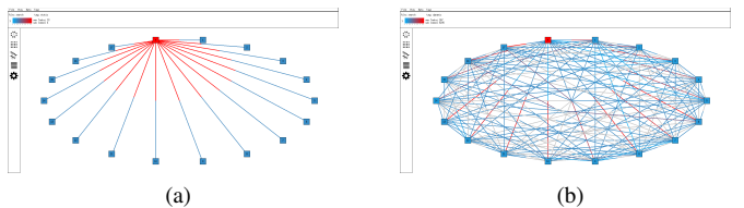
Fig. 11. Output of Chplvis [18] for (a) static load distribution (b) Dynamic distributed iterator. Results are for size N = 18 running on 16 locales. In the figure, when the color of an edge \{x, y\} is red closer to x means that much more communication happen from x to y rather than y to x .
