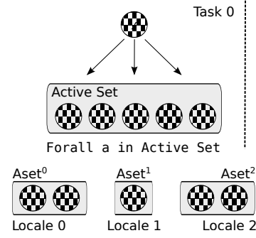
Fig. 3. Task 0 is responsible for distributing the active set across several locales. The distributed active set A_d consists of several sets A_d^i , i \in \{0, \dots, l-1\} , where l is the number of locales on which the application is going to run.
