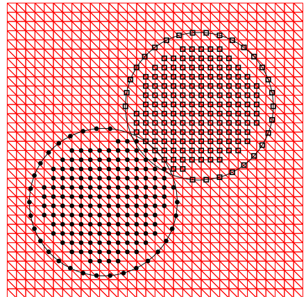
Fig. 2: DLM/FD set of points for two colliding circular particles
