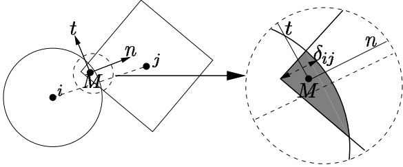
Fig. 1: Contact between two particles: i and j denote gravity center of particles i and j respectively, M the contact point, n and t unit normal and tangential vectors at the contact point respectively and \delta_{ij} the overlapping distance
