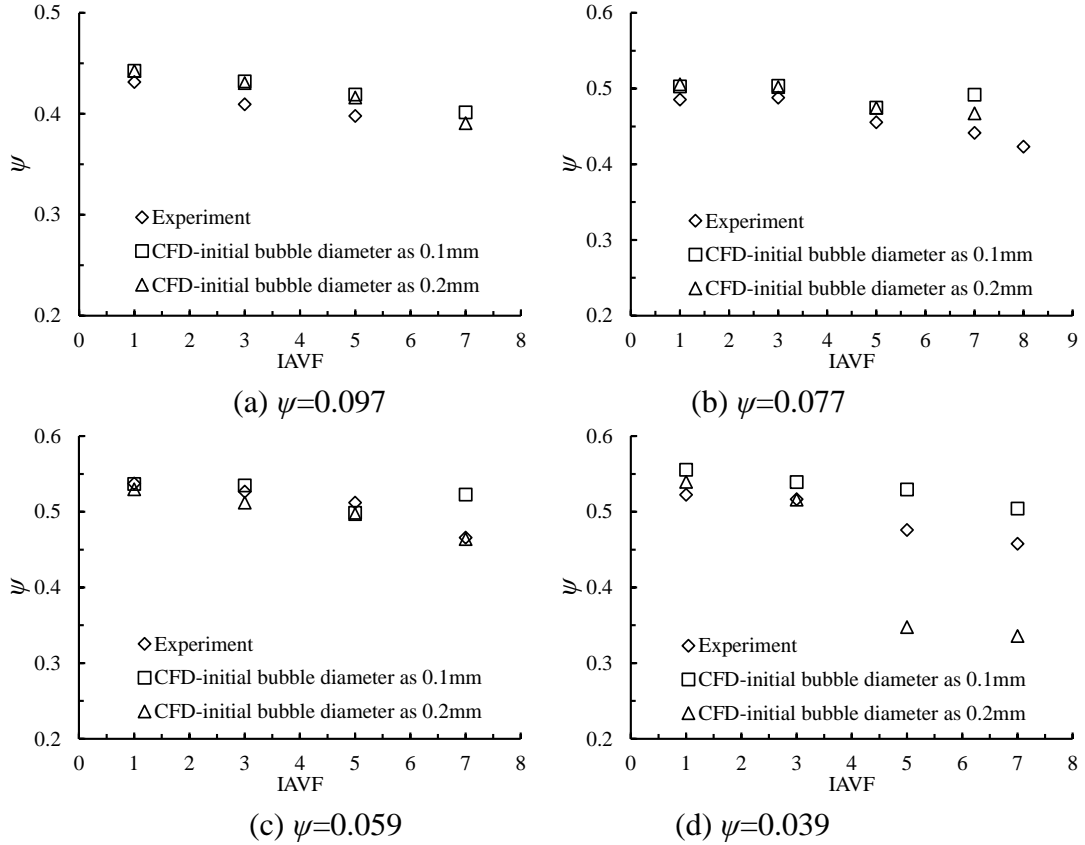
Figure 6: Comparisons of head pump coefficient for different IAVF values
