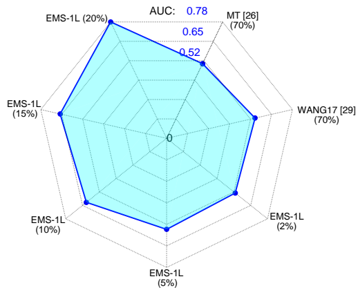
Figure 4: Comparison of the classification accuracy of EMS-1L, using different amounts of labelled data, against state-of-the-art methods.
