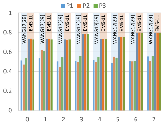
Figure 3: Plot highlighting the sensitivity of the AUC for each class when changing the data partition of the data set (using 15% for training)
