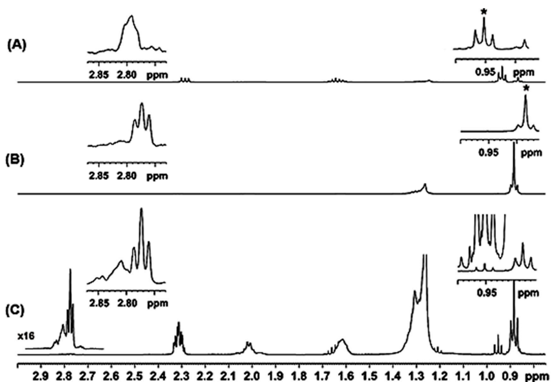
Figure 2. (A) Selected region of a 500 MHz 1 H-NMR spectrum of the lipid fraction of a lyophilized bovine milk sample in CDCl 3 ; T, 298 K; number of scans, 256; acquisition time, 4.3 s; relaxation delay, 5 s; total experimental time ~25 min. (B) and (C) 1D TOCSY spectra with τ m = 200 ms, number of scans, 256 and total experimental time ~25 min. The asterisks (*) denote the -CH 3 resonances that were excited with the use of a selective shaped pulse of 80 ms.
