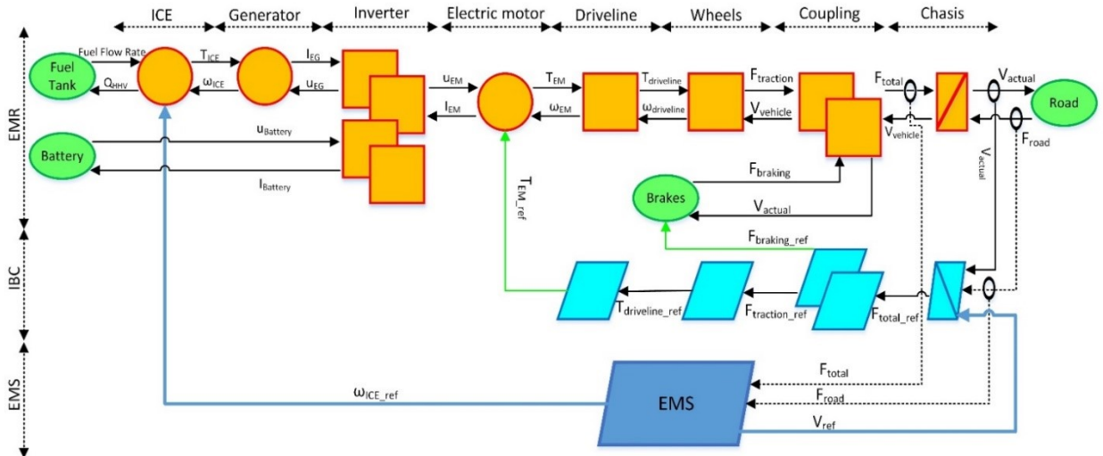
Figure 2: Energetic Macroscopic Representation and Inversion-Based Control of the investigated series hybrid powertrain
