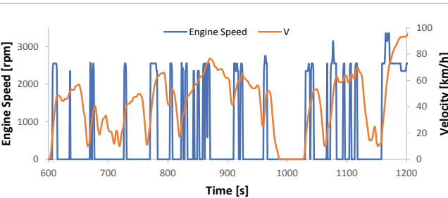
Figure 9: Optimal engine speed for part of the first WLTP cycle.
