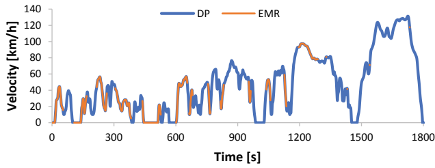
Figure 6: Vehicle speed profile validation between DP and EMR models.
