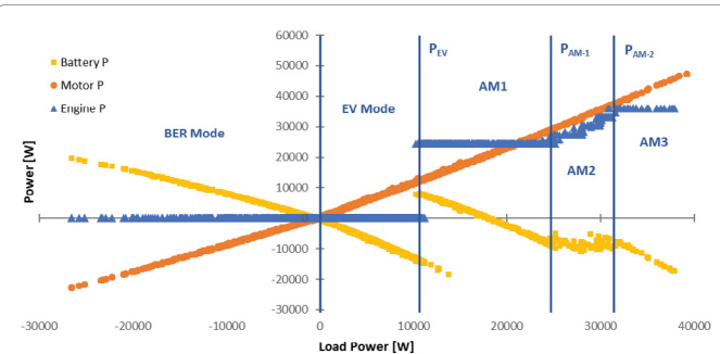
Figure 11: Power behavior of the drivetrain components under DP control for three repeated WLTPs.
