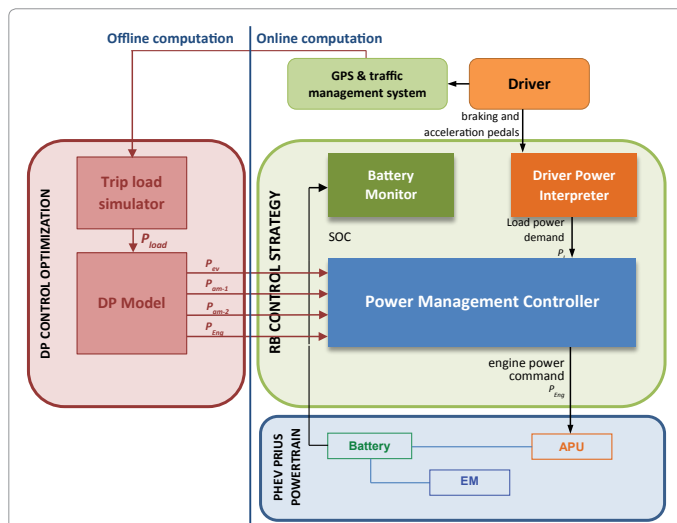
Figure 13: Optimized rule based EMS architecture of Series PHEV.
