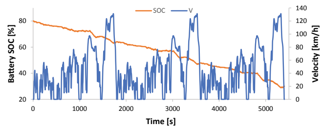
Figure 10: Optimal battery SOC path for three repeated WLTPs.
