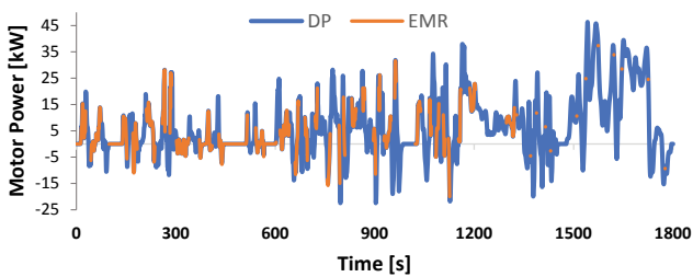
Figure 8: Electric motor power profile validation between DP and EMR models.
