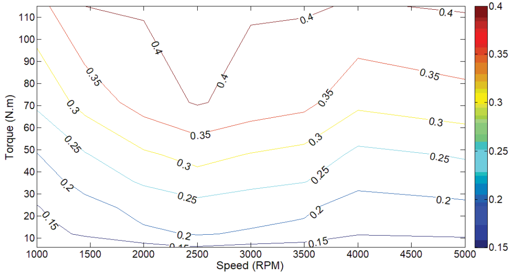
Figure 4: Engine efficiency map.
