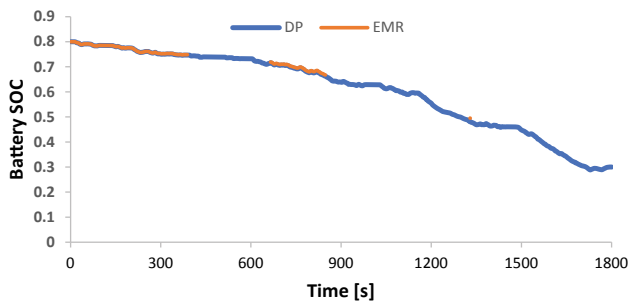
Figure 7: Battery SOC profile validation between DP and EMR models.
