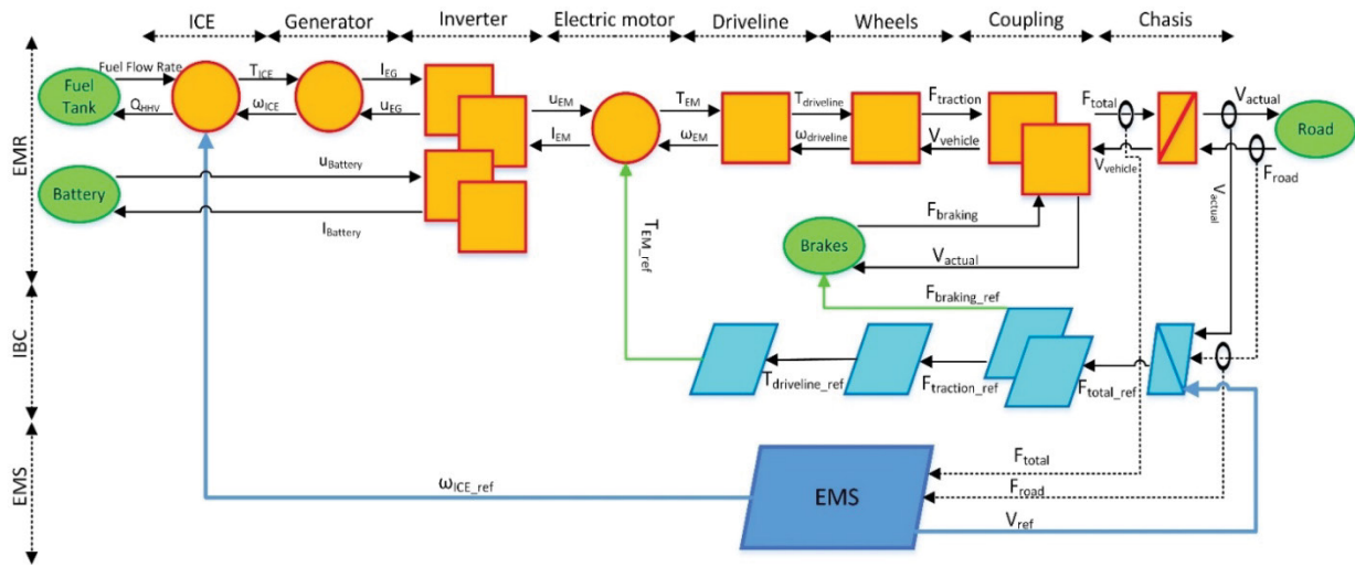
Figure 3: Energetic macroscopic representation and inversion-based control of the investigated series hybrid powertrain.
