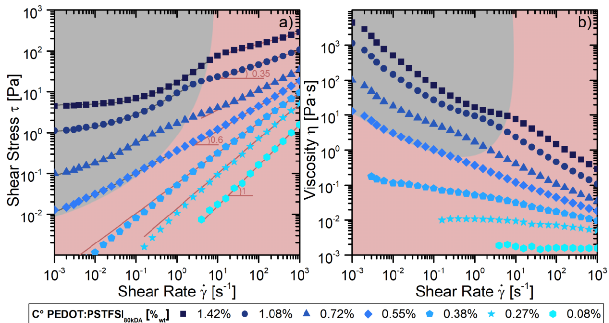
Figure 1. Rheological behavior of PEDOT:PSTFSI inks measured with a shear rheometer (cone plate geometry: 50 mm diameter and 1^\circ angle): a) shear stress versus shear rate and b) viscosity versus shear rate obtained by applying shear rate ramps at 18^\circ\text{C} . The lines are fits to the data using the power model (red) or the HB model (grey). The numbers are the values of the parameter n .
