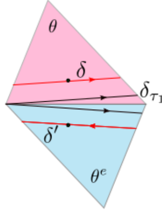
FIGURE 24. Two neighbouring tiles \theta and \theta^e and trajectories \delta and \delta' passing by circumcenters of the tiles. The trajectory \delta_{\tau_1} is a periodic loop containing e .
