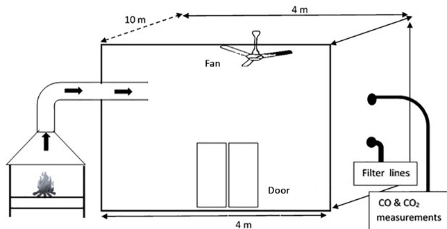
Figure 2. Schematic view of the Lannemezan combustion chamber.
