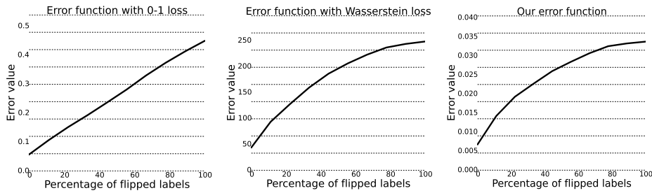
Fig. 1: Comparison of empirical error functions defined with (left) traditional 0-1 loss, (middle) original Wasserstein loss and (right) global error function from this paper. The errors were averaged based on class probabilities obtained by fitting a linear classifier on samples consisting of 500 to 10500 instances with step equal to 1000 with 20 features and 2 classes. The classification problem is made gradually harder by randomly flipping a certain proportion of instances' labels (x-axis) between the two classes. For the original Wasserstein loss, we calculate point-wise Wasserstein distances between the vector of probabilities and the one-hot encoding vector with the true label. For our error function, we calculate the Wasserstein distance between the normalized vectors of probabilities over all instances and that of true labels. We observe that despite the different scales, all losses behave similarly and reflect the increasing difficulty of the classification problem.
