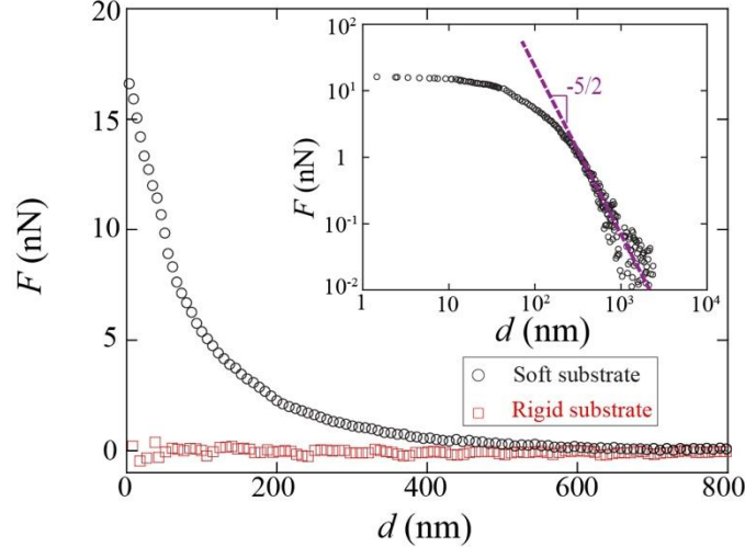
Figure 2. Temporal average F of the normal force F_N (see Fig.1) as a function of the gap distance d to the substrate, for both rigid (silicon wafer) and soft (PDMS 20:1) substrates. The liquid used is PDMS oil with viscosity \eta=9.3 \text{ mPa} \cdot \text{s} . The amplitude of the velocity is A\omega = 5.75 \text{ mm/s} . The inset shows a log-log representation of the data for the soft substrate, and the solid line therein indicates a -5/2 power law.
