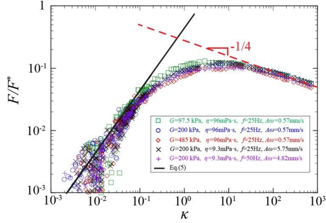
Figure 4. Dimensionless force F/F^* as a function of dimensionless compliance \kappa (see definitions in text) in logarithmic scales, as measured from force-distance data (see Figs.2 and 3), for all the experiments performed in this study (see Fig.3). The solid line corresponds to the theoretical prediction for F at low \kappa , obtained from Eq.(5) where V is replaced by A\omega/\sqrt{2} due to the temporal averaging step. The dashed lined indicates a -1/4 power law.
