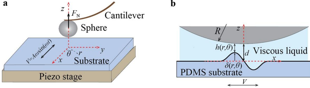
Figure 1. Schematic of the experimental setup. The soft PDMS sample is fixed to a rigid piezo stage that is transversally oscillated along time t , at angular frequency \omega , and with amplitude A . A rigid borosilicate sphere is glued to an AFM cantilever and placed near the substrate, with silicon oil or PDMS oil as a viscous liquid lubricant. The normal force F_N exerted on the sphere, at a gap distance d from the surface, is directly measured from the deflection of the cantilever.
