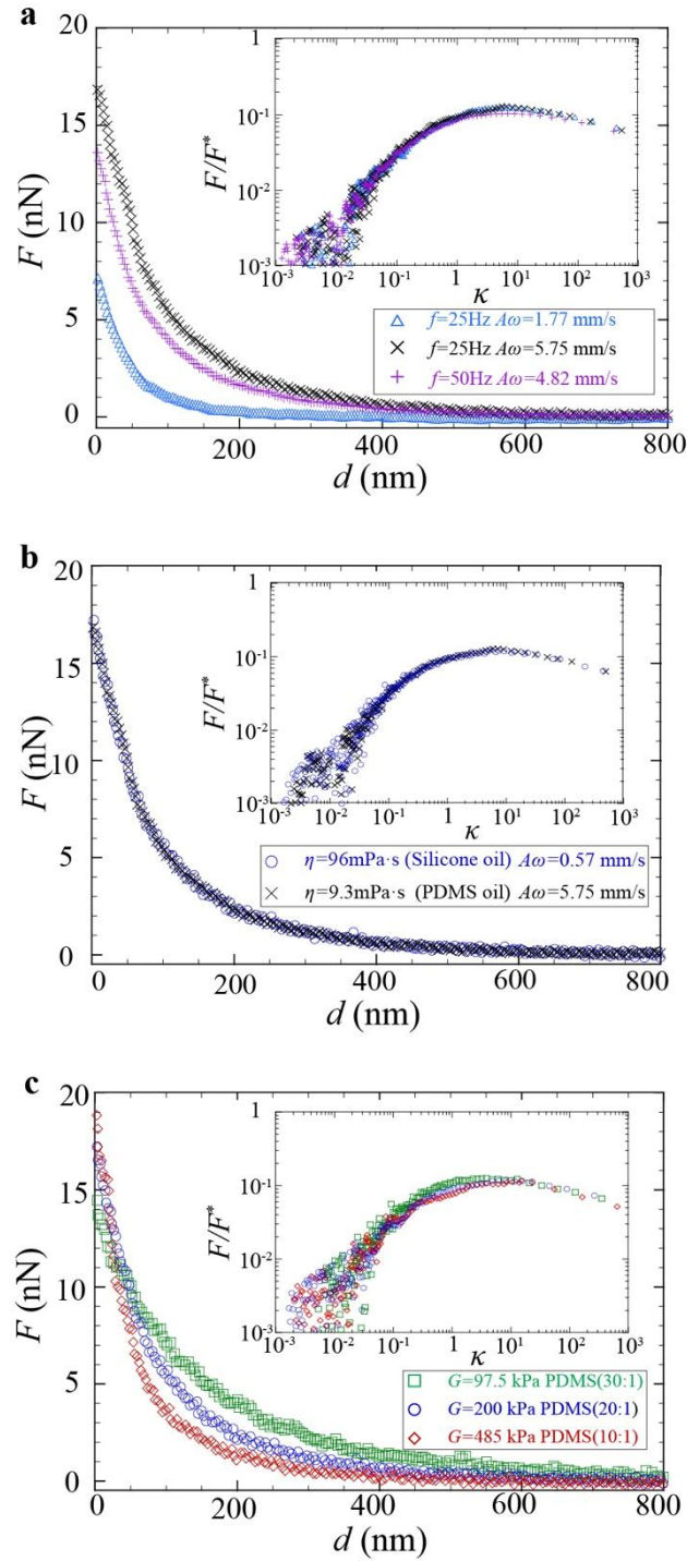
Figure 3. Measured temporal-averaged force F as a function of gap distance d to the soft PDMS substrates, and (insets) dimensionless force F/F^* as a function of dimensionless compliance \kappa in logarithmic scales, for various sets of parameters. (a) three different velocity amplitudes (as indicated) are investigated. The substrate is crosslinked PDMS (20:1), and the liquid is PDMS oil with viscosity \eta = 9.3 mPa \cdot s; (b) two different liquid and associated viscosities (as indicated) are investigated. The substrate is crosslinked PDMS (20:1), and the velocity amplitudes are A\omega = 0.57 mm/s and A\omega = 5.75 mm/s for silicone oil ( \eta = 96 mPa \cdot s) and PDMS oil ( \eta = 9.3 mPa \cdot s) respectively. (c) three different shear moduli (as indicated) of the substrate are investigated. The liquid is silicone oil with viscosity \eta = 96 mPa \cdot s, and the velocity amplitude is A\omega = 0.57 mm/s.
