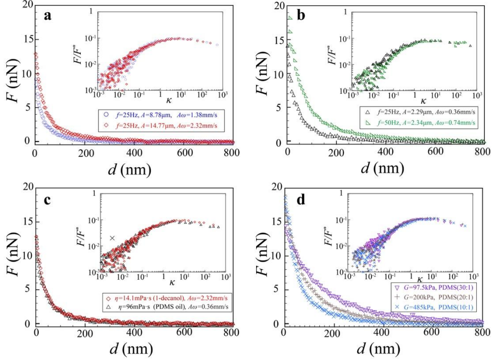
Figure 3. Measured temporal-averaged force F as a function of gap distance d to the soft PDMS substrates, and (insets) dimensionless force F/F^* as a function of dimensionless compliance \kappa in logarithmic scales, for various sets of parameters. (a) Two different velocity amplitudes (as indicated) obtained with different oscillation amplitudes are investigated. The substrate is crosslinked PDMS (10:1), and the liquid is 1-decanol with viscosity \eta = 14.1 \text{ mPa} \cdot \text{s} ; (b) two different velocity amplitudes (as indicated) obtained with two different working frequencies are investigated. The substrate is crosslinked PDMS (10:1), and the liquid is silicone oil with viscosity \eta = 96 \text{ mPa} \cdot \text{s} ; (c) two different liquids with different associated viscosities (as indicated) are investigated. The substrate is crosslinked PDMS (10:1), and the velocity amplitudes are A\omega = 0.36 \text{ mm/s} and A\omega = 2.32 \text{ mm/s} for silicone oil ( \eta = 96 \text{ mPa} \cdot \text{s} ) and 1-decanol ( \eta = 14.1 \text{ mPa} \cdot \text{s} ) respectively; (d) three different shear moduli (as indicated) of the substrate are investigated. The liquid is silicone oil with viscosity \eta = 96 \text{ mPa} \cdot \text{s} , and the velocity amplitude is A\omega = 0.57 \text{ mm/s} .
