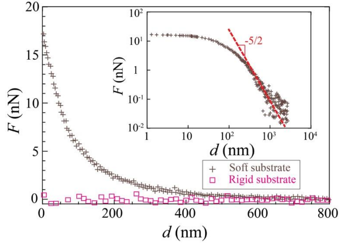
Figure 2. Temporal average F of the normal force F_N (see Fig.1) as a function of the gap distance d to the substrate, for both rigid (silicon wafer) and soft (PDMS 20:1) substrates. The liquid used is silicone oil with viscosity \eta=96 \text{ mPa} \cdot \text{s} . The amplitude of the velocity is A\omega = 0.57 \text{ mm/s} . The inset shows a log-log representation of the data for the soft substrate, and the solid line therein indicates a -5/2 power law.
