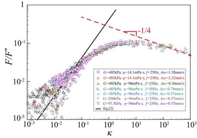
Figure 4. Dimensionless force F/F^* as a function of dimensionless compliance \kappa (see definitions in text) in logarithmic scales, as measured from force-distance data (see Figs.2 and 3), for all the experiments performed in this study (see Fig.3). The solid line corresponds to the theoretical prediction for F at low \kappa , obtained from Eq.(2) where V is replaced by A\omega/\sqrt{2} due to the temporal averaging step. The dashed lined indicates a -1/4 power law.
