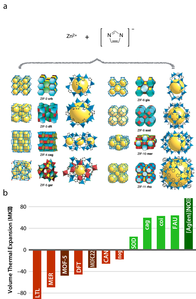
Figure 4: (a) The molecular components of ZIFs which can generate diverse structural topologies. (b) Thermal expansion coefficients of ZIF frameworks with varying topology (LTL, MER, DFT, CAN, nog, SOD, cag, coi, and FAU). Values for some other MOFs are reported for comparison: MOF-5, MOF-C22, and [Ag(en)]NO 3 . Reproduced with permission from Ref. 42 and Ref. 41
