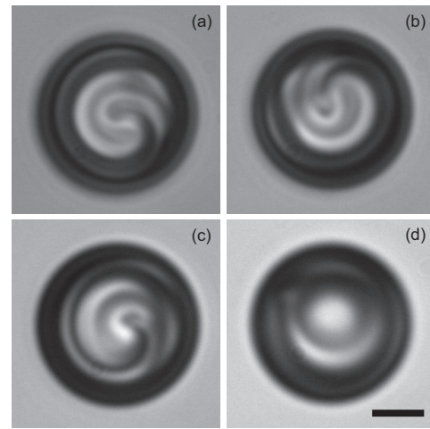
Fig. 6 The same spiraling droplet at four different temperature gradients: (a) \Delta T = 1^\circ\text{C} ; (b) \Delta T = 3^\circ\text{C} ; (c) \Delta T = 5^\circ\text{C} and (d) \Delta T = 9^\circ\text{C} , for the same average temperature of 27.5^\circ\text{C} . At the larger temperature gradient, the contrast has changed significantly, meaning that the texture was distorted. The black bar is 10 \mu\text{m} long.
