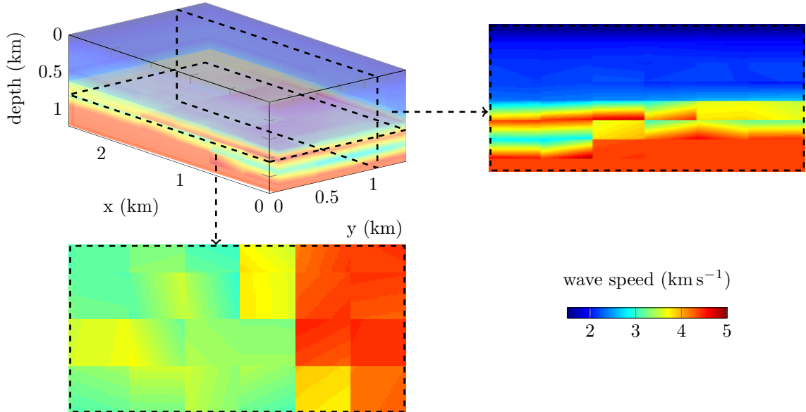
Figure 8: Illustration of the unstructured tetrahedral mesh of the model, using 433 979 tetrahedra.
