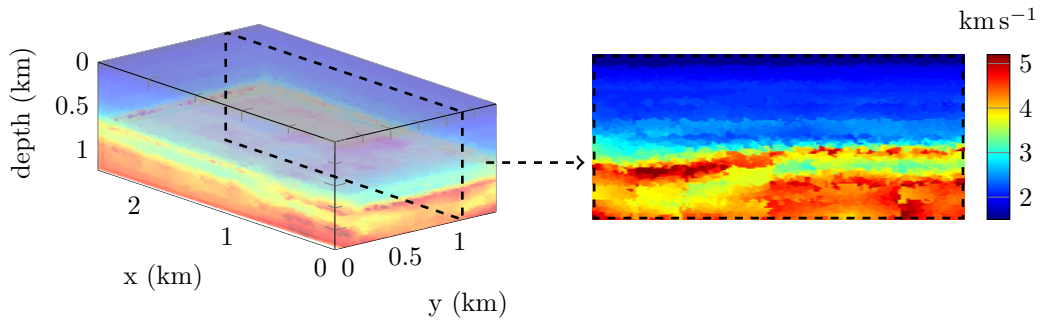
Figure 14: Three-dimensional representation and vertical section at y = 1.125\text{km} of the reconstruction from 10Hz Cauchy data after 175 iterations. The partition consists of N = 1089 subdomains, leading to a total number of unknowns of 4 \times 1089 = 4356 . The initial model varies in depth only and is shown in Figure 13. The relative L^2 difference with the reference model Figure 3 is \mathcal{E}_{\text{rel}} = 0.119 .
