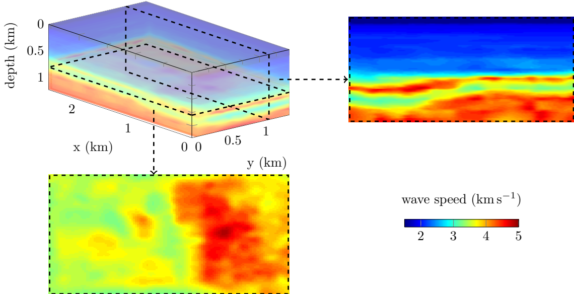
Figure 11: Three-dimensional representation and vertical section at y = 1.125\text{km} of the reconstruction from 10Hz Cauchy data after 175 iterations. The partition consists of N = 1089 subdomains, leading to a total number of unknowns of 4 \times 1089 = 4356 . The initial model is shown in Figure 10.
