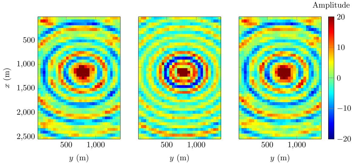
(a) Fourier transform of the time-domain observation. (b) Simulated data using the initial model of Figure 13. (c) Simulated data from the reconstructed model Figure 14.
