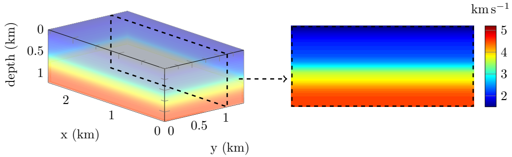
Figure 13: Three-dimensional representation and vertical section at y = 1.125\text{km} of the initial model, which varies in depth only.
