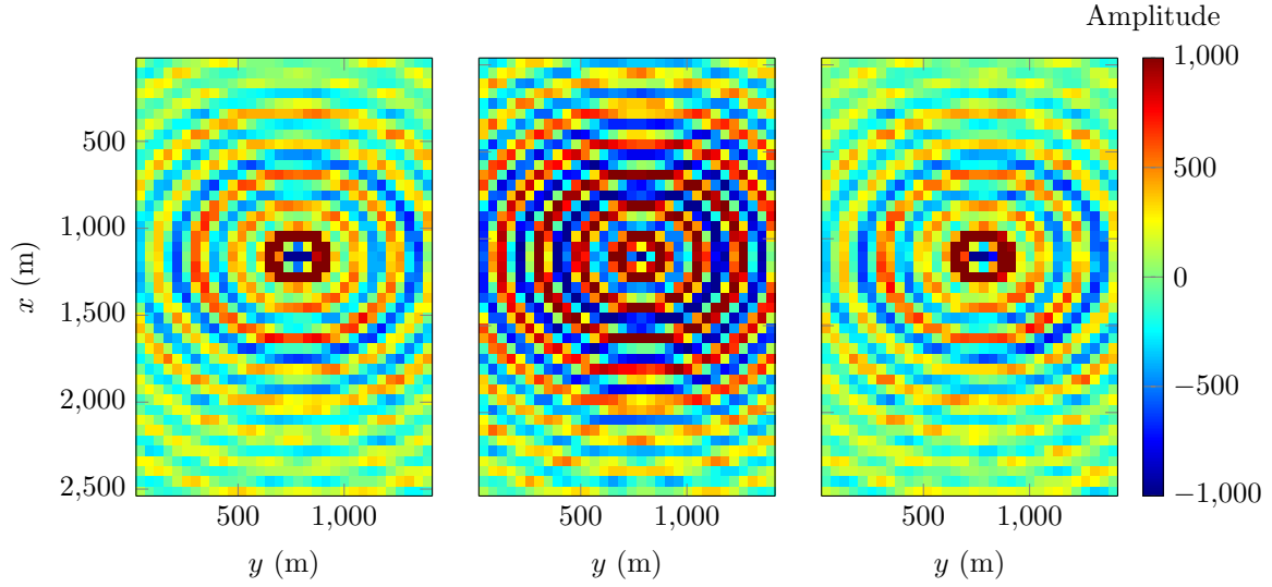
(a) Fourier transform of the time-domain observation. (b) Simulated data using the initial model of Figure 13. (c) Simulated data from the reconstructed model Figure 14.
