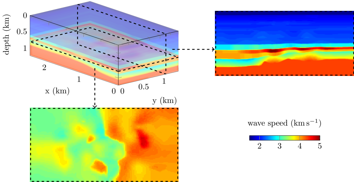
Figure 3: Three-dimensional representation, horizontal section at 800m depth and vertical section at y = 1.125\text{km} of the reference wave speed. It is represented with 1 527 168 nodal values.
