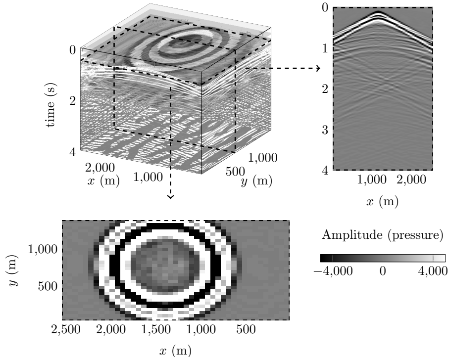
Figure 5: Three-dimensional time-domain pressure trace for a centrally located source. Sections at fixed time t = 0.5\text{s} and for a fixed line of receivers positioned in y = 695\text{m} are respectively given at the bottom and right of the 3D visualization. The x and y axis correspond with the receivers map ( i.e. , every 60m for x and 45m for y ).
