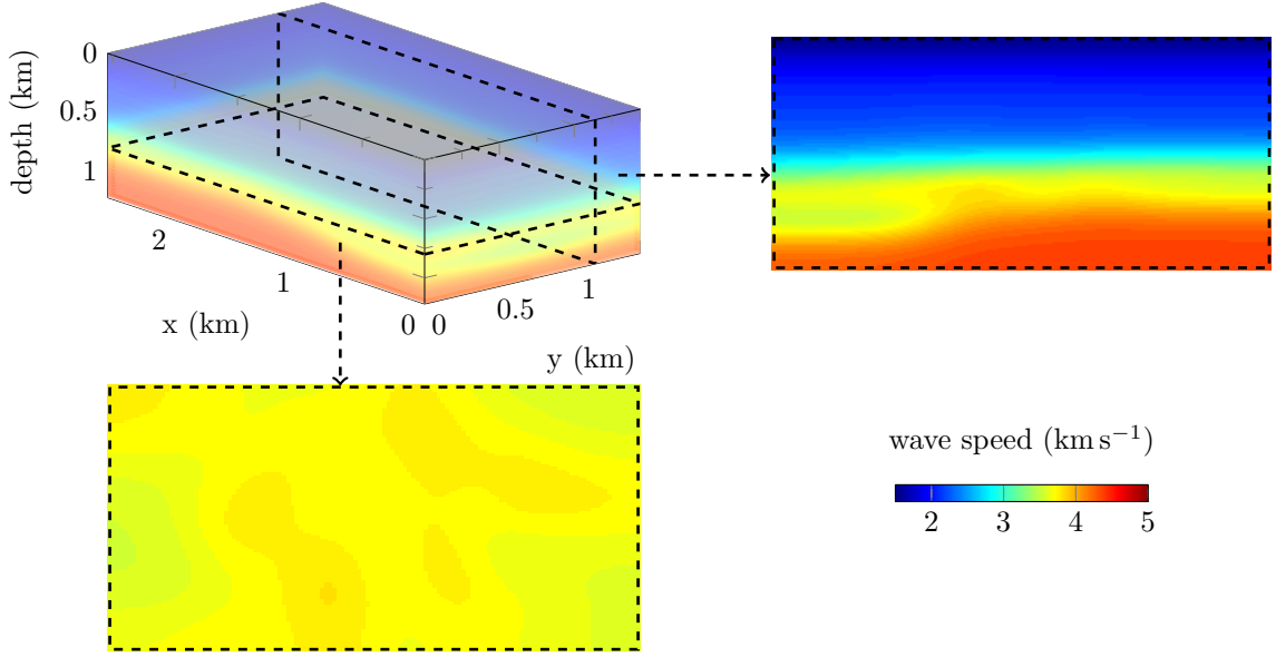
Figure 10: Three-dimensional representation, horizontal section at 800m depth and vertical section at y = 1.125\text{km} of the initial wave speed model.
