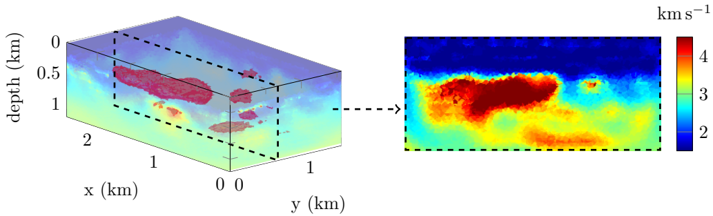
Figure 21: Three-dimensional representation and vertical section at y = 670\text{m} of the reconstruction using 4Hz Cauchy data after 100 iterations and where the simulation setup differs from the original measurement acquisition, see Table 1. The relative L^2 difference with the reference model Figure 19 is \mathcal{E}_{\text{rel}} = 0.174 .
