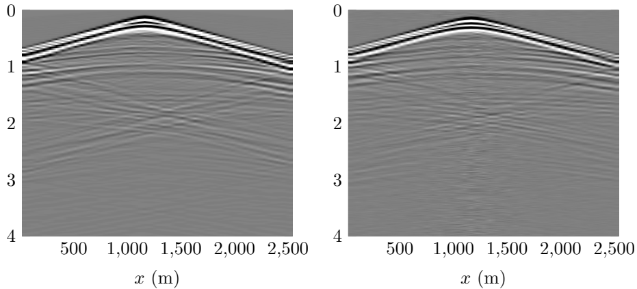
(a) Noiseless synthetic trace section.
