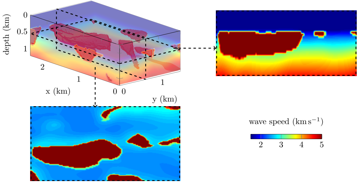
Figure 19: Three-dimensional representation, horizontal section at 550m depth and vertical section at y = 670\text{m} of the reference wave speed encompassing salt domes. The wave speed in the domes is a constant of 4500\text{m s}^{-1} .
