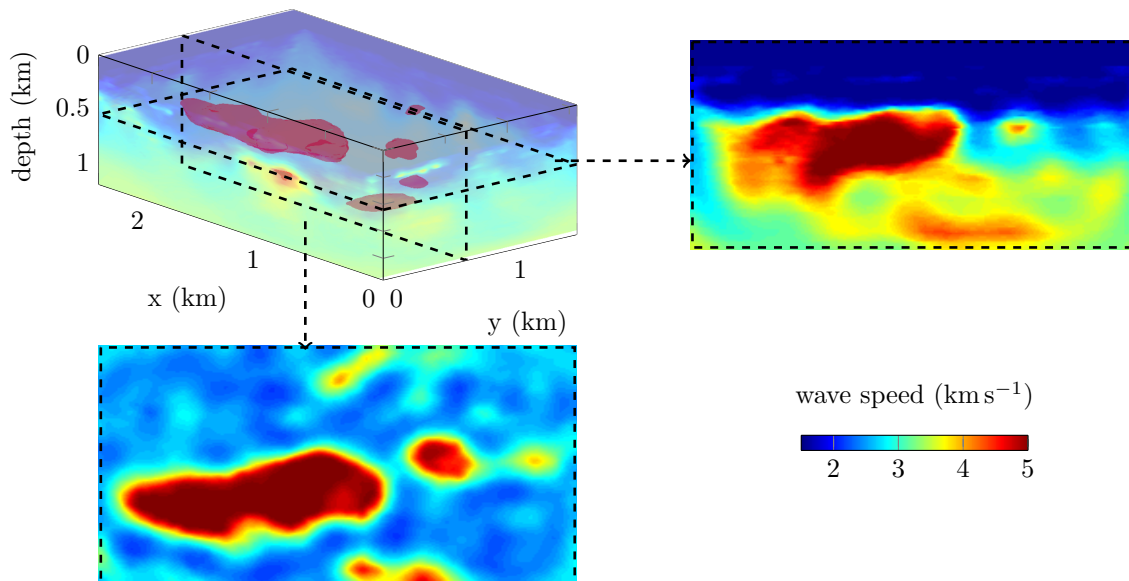
Figure 22: Gaussian filtering (see Remark 2) of the reconstruction (Figure 21) obtained using 100 iterations with 4Hz Cauchy data and where the setup for simulation differs from the original measurement acquisition. Three-dimensional representation, horizontal section at 550m depth and vertical section at y = 670\text{m} . The relative L^2 difference with the reference model Figure 19 is \mathcal{E}_{\text{rel}} = 0.172 .
