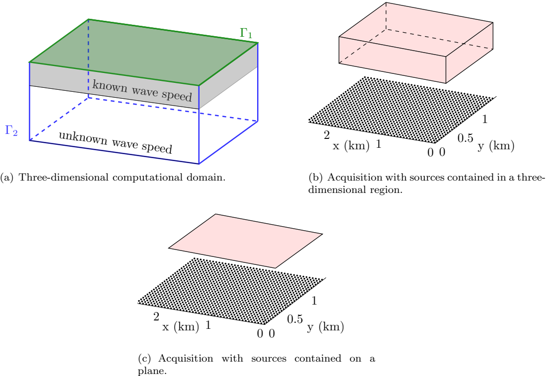
Figure 4: Illustration of the configuration. (a) We apply a Dirichlet boundary on the upper surface \Gamma_1 (in green) and absorbing boundary conditions on \Gamma_2 = \partial\Upsilon \setminus \bar{\Gamma}_1 (indicated in blue). (b)–(c) The sources that probe the Cauchy data lie in between the receivers and the free surface. Sources are positioned in a three or two-dimensional region (in red). The position of the receivers (black dots) remains fixed. Both receivers and sources lie in the area of known wave speed.
