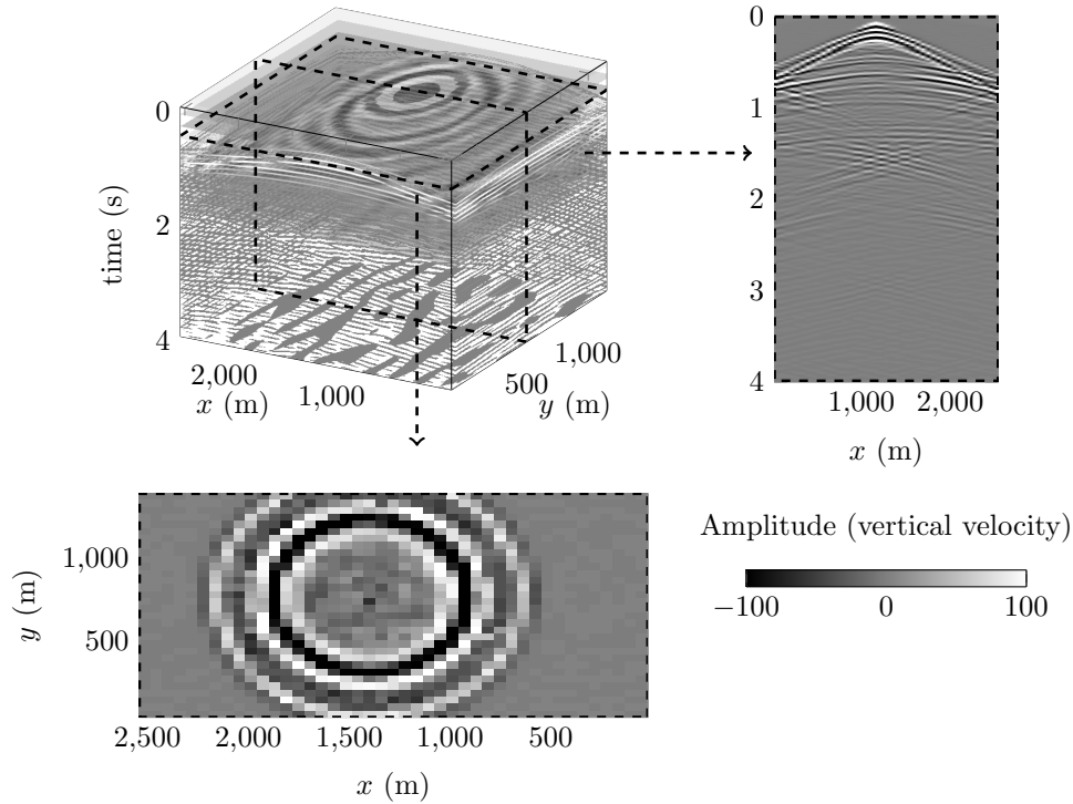
Figure 6: Three-dimensional time-domain vertical velocity trace for a centrally located source. Sections at fixed time t = 0.5\text{s} and for a fixed line of receivers positioned in y = 695\text{m} are respectively given at the bottom and right of the 3D visualization. The x and y axis correspond with the receivers map ( i.e. , every 60m for x and 45m for y ).
