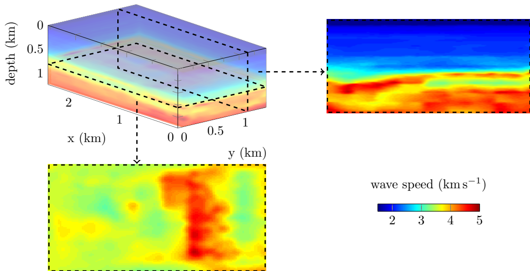
Figure 15: Gaussian filtering (see Remark 2) of the reconstruction (Figure 14) obtained from 10Hz Cauchy data starting with the initial model that varies in depth only (Figure 13). Three-dimensional representation, horizontal section at 800m depth and vertical section at y = 1.125\text{km} . The relative L^2 difference with the reference model Figure 3 is \mathcal{E}_{\text{rel}} = 0.108 .
