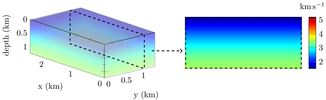
Figure 20: Three-dimensional representation and vertical section at y = 670\text{m} of the initial model, which varies in depth only.
