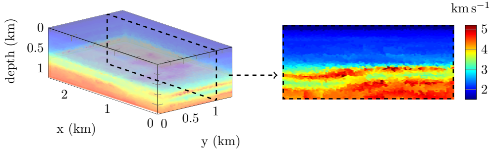
(a) Reconstruction where the sources in the acquisition are positioned in a three-dimensional area (see Figure 4(b)); the relative L^2 difference with the reference model Figure 3 is \mathcal{E}_{\text{rel}} = 0.083 .
