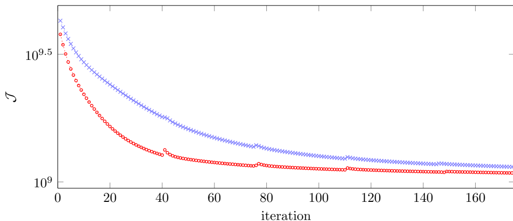
Figure 16: Evolution of the misfit functional with iterations, the blue crosses correspond with the case where the initial model is one-dimensional (see Figure 13 for the initial model and Figure 14 for the associated reconstruction); the red circles correspond with the case where the initial model is smooth (see Figure 10 for the initial model and Figure 11(b) for the associated reconstruction).
