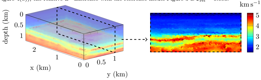
(b) Reconstruction where the sources in the acquisition are limited on a plane (see Figure 4(c)); the relative L^2 difference with the reference model Figure 3 is \mathcal{E}_{\text{rel}} = 0.088 .
