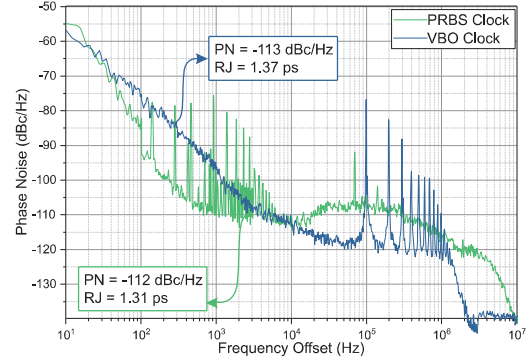
Fig. 7. Phase noise of VBO and PRBS clock.
