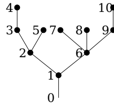
Associated genealogical height process \mathcal{H} .
