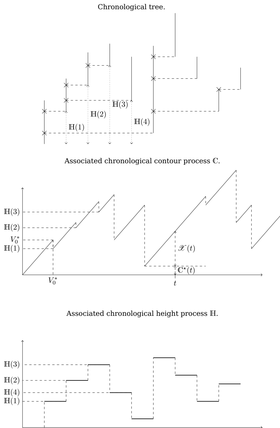
Figure 4: Chronological height and contour processes associated with the chronological tree constructed from the sequence of sticks of Figure 1.
