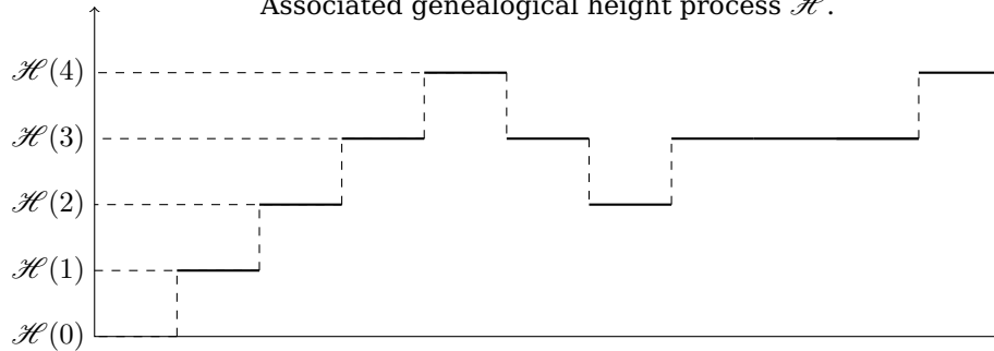
Associated genealogical height process \mathcal{H} .
