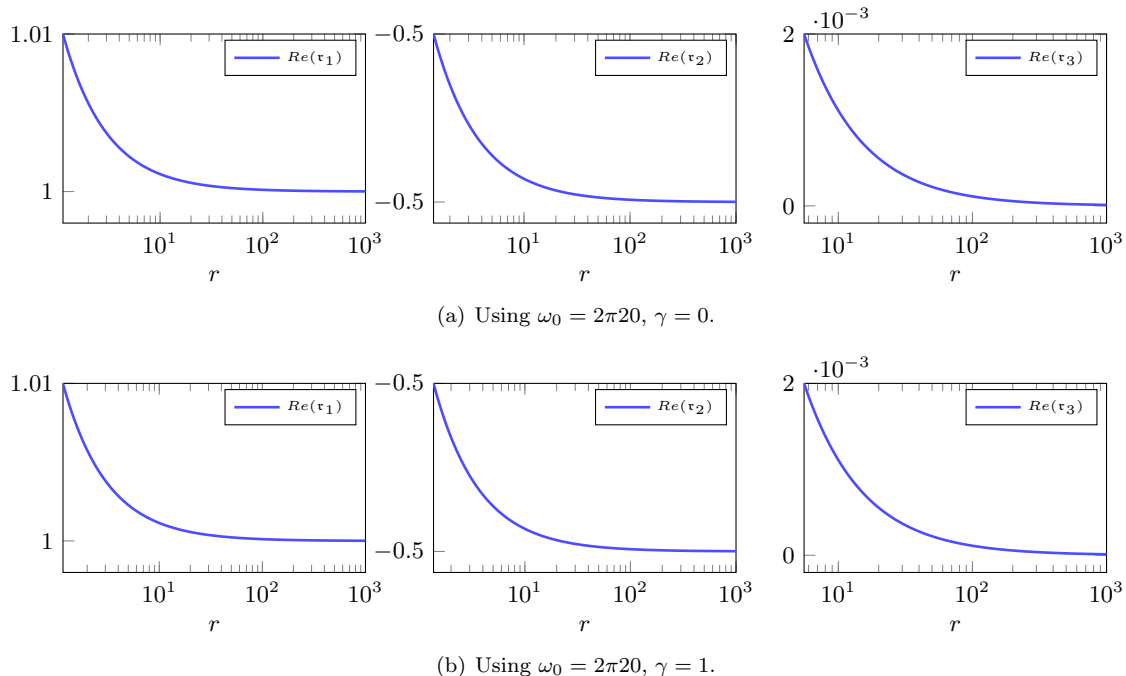
Figure 7: Plots of ratios (4.52) which represent the symbol part of W_{-i\eta, 1/2}(-2ikr) , its derivative and the radiating property. These are the remainder after the oscillatory part \exp(\varphi_k(r)) defined in (4.51) is factored out from the functions. The curves show that they all have the profile of a constant +o(1) , thus have horizontal asymptotes given by the leading constants. The horizontal asymptote for \tau_1 is 1, while that for its derivative is -1/2 . As a result, that for W_{-i\eta, 1/2}(-2ikr)' + \frac{1}{2}W_{-i\eta, 1/2}(-2ikr) is 0.
