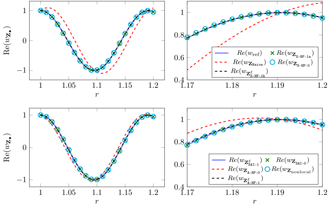
Figure 13: Comparison of w_{\mathbf{z}_\bullet} solution to (6.39) on [1, 1.2] with the analytical solution w_{\text{ref}} in (6.41). Here the comparison is in terms of the real part of the solution. The parameters used are \omega_0 = 2\pi 20 , \alpha_\infty = 50 , l = 3 and \gamma = 0 . Evolution of the global profile (left) and zoom towards the end (right).
