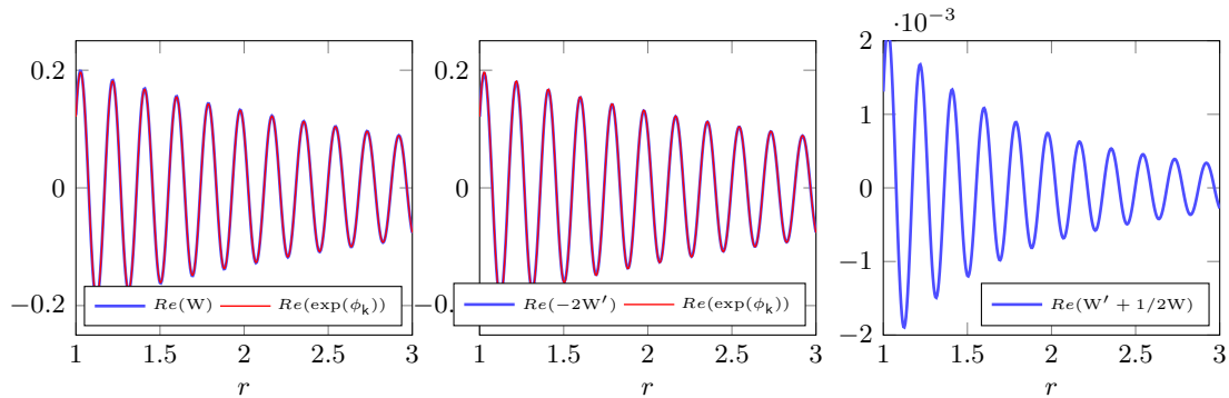
Figure 6: Outgoing Whittaker function W_{-i\eta, 1/2}(-2ikr) in the case with attenuation ( \gamma = 1 ) at frequency \omega_0 = 2\pi 20 . The leading part in the asymptotic is given by e^{\varphi_k(r)} where \varphi_k(r) := ikr - i\eta \log(2kr) - \frac{\pi}{2}\eta , and \eta = \frac{\alpha}{2k} with c = 3 and \alpha = 50 , see (4.45). Here, the oscillatory behavior is now coupled with attenuation which translates to a decrease in magnitude of the oscillating curve. The function \exp(\varphi_k(r)) still represents an excellent approximation as in the case without attenuation.
