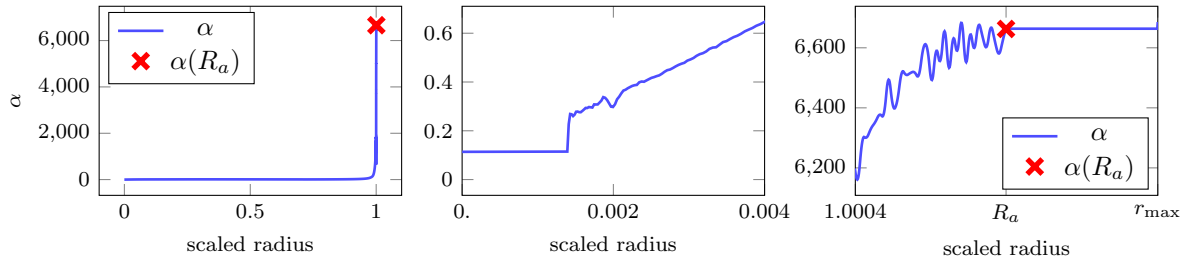
Figure 2: Profile of the inverse of density scale-height \alpha from (2.10) in the model \mathbf{S+Atmo} shown on the whole interval r \leq r_{\max} (on the left) and zoomed (on the right) near R_a . This plot shows that \alpha is positive and is constant for r \geq R_a . In addition, near r = 0 , \alpha is strictly positive, which means that the resulting potential \mathbf{q} (2.11) not only has a Coulomb-type potential but also a weak-singularity at r = 0 , cf. (2.15) and (2.16).
