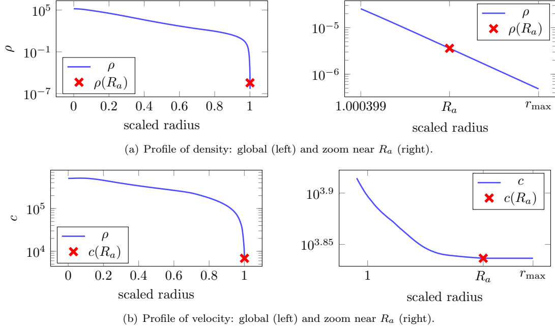
Figure 1: Profile of density and velocity in the model \mathbf{S+Atmo} on r \leq r_{\max} = 1.001 . The interior of the Sun, r < R_a = 1.000699 , is described by model \mathbf{S} [8] and extended into the atmosphere by (2.13).
