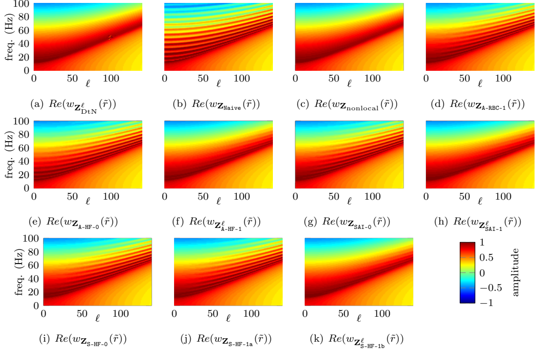
Figure 15: Comparison of the solutions Re(w_{\bullet, \ell, \omega_0}(\tilde{r})) as a function of the frequency \omega_0 and \ell in \tilde{r} = 1.01 without attenuation ( \gamma = 0 ).
