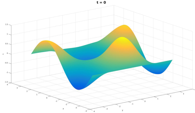
FIGURE 1. Initial data (14)
