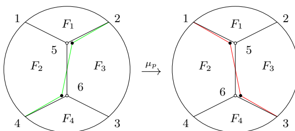
Fig. 2: An oriented flip graph
