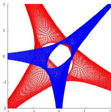
Fig. 2: The intersection of f_1(z_1, z_2) := z_1^2 z_2^2 + z_1 z_2 + z_1 + z_2 and f_2(z_1, z_2) := z_1^3 + z_2^3 + 2z_1 z_2 + 1 . None of the vertices of \mathcal{I}(\{f_1, f_2\}) given by the intersection of the boundaries of the two bounded components of the complement of \mathcal{A}(f_1) and \mathcal{A}(f_2) are vertices of the corresponding intersection polytopes.
