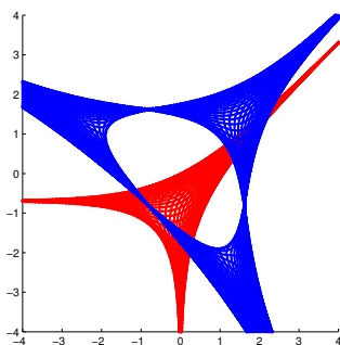
Fig. 1: An approximation of the amoebas \mathcal{A}(f_1) and \mathcal{A}(f_2) for f_1 := 2z_1 + z_2 + 1 and f_2 := z_1^2 z_2 + z_1 z_2^2 + 5z_1 z_2 + 1 . The intersection \mathcal{A}(f_1) \cap \mathcal{A}(f_2) consists of two connected components.
