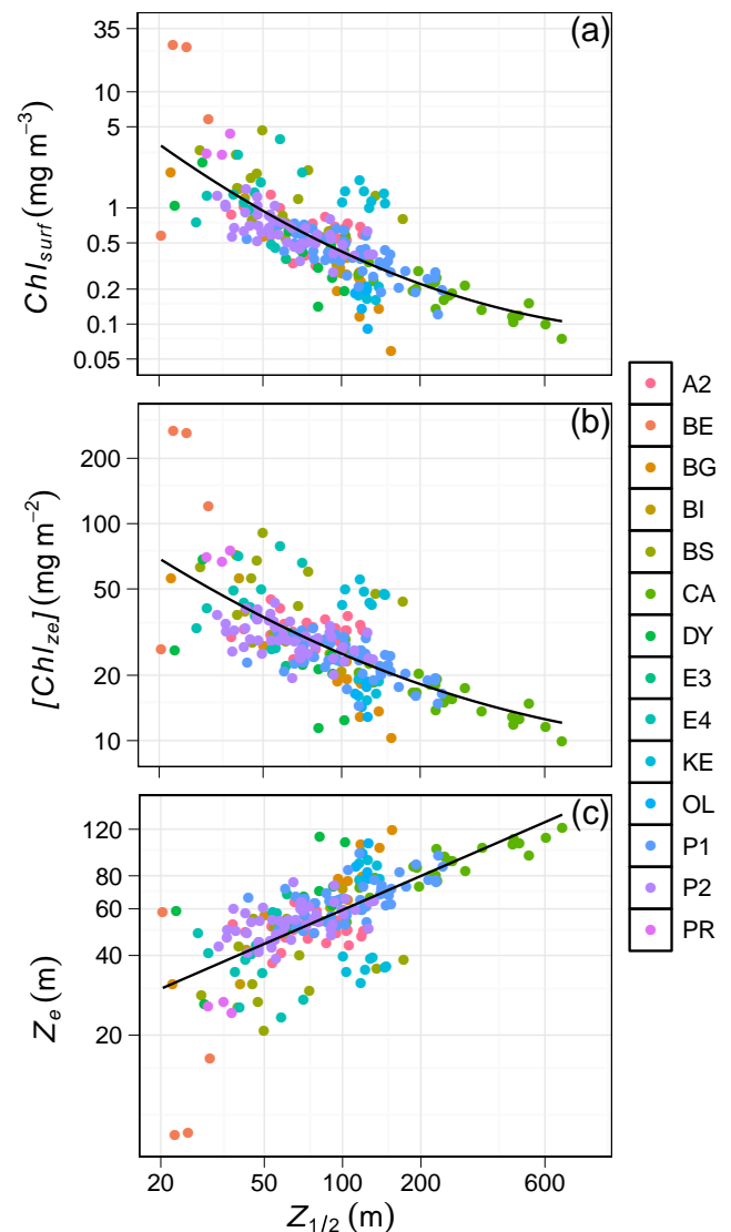
Fig. 5. Sigmoid profiles: Scatterplot of \log_{10} -transformed \text{Chl}_{\text{surf}} ( \text{mg m}^{-3} ), [\text{Chl}_{ze}] ( \text{mg m}^{-2} ) and Z_e (m) as a function of \log_{10} -transformed depth-dependent shape parameter Z_{1/2} (m). Colors refer to the different cruises/projects (see Table 2 for the abbreviations). The line is the polynomial fit within the data. The order of this fit as well as the coefficient of determination and the residuals standard error are indicated in Table 4.
