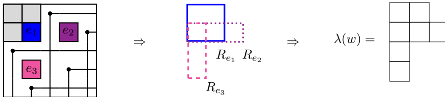
Fig. 1: The diagram of w = 35142 (with color coded essential set \{e_1, e_2, e_3\} ), the overlay of R_{e_1}, R_{e_2}, R_{e_3} , and the shape \lambda(w) .
