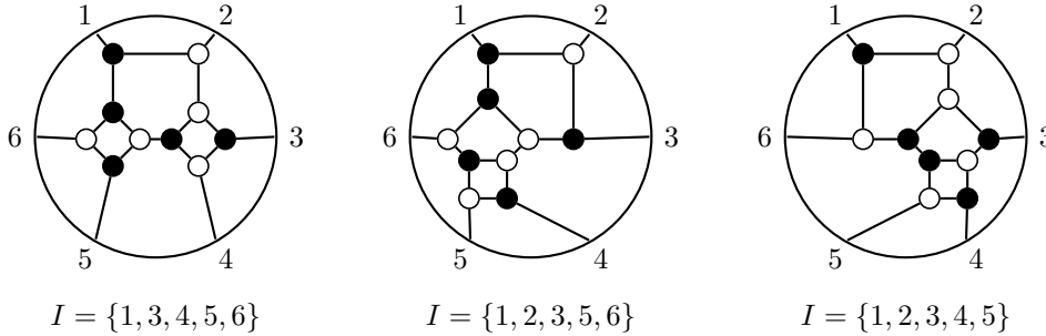
Fig. 1: The (1+2,6) -scattering amplitude to zeroth order can be expressed as a sum of three terms, arising from the three on-shell diagrams, or plabic graphs, shown, which we obtain by the BCFW recursion. These graphs label cells of \text{Gr}_{3,6}^{\geq 0} , and there is a further step (which we do not discuss here) which decreases the index k by 2, giving three cells of \text{Gr}_{1,6}^{\geq 0} , each indexed by a subset of [6] . The images of these cells under Z in \text{Gr}_{1,5} triangulate the amplituhedron \mathcal{A}_{6,1,4}(Z) (for general k, n this is only conjecturally true), using which the sum of 3 terms can be collapsed into a single integral over \mathcal{A}_{6,1,4}(Z) .
