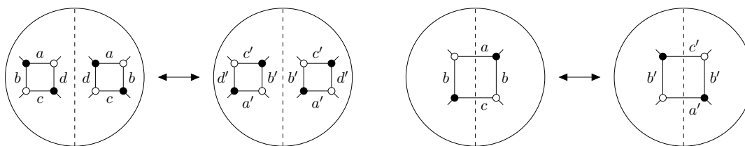
(a) Two of Postnikov's moves combine to give a symmetric local move.
