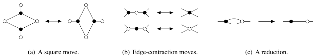
Fig. 2: Moves and reductions for plabic graphs.
