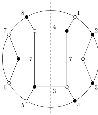
Fig. 1: A symmetric weighting of a symmetric plabic graph. All unlabeled edges have weight 1.
