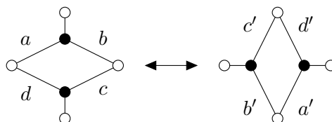
Fig. 3: A square move gives a change of coordinates.
