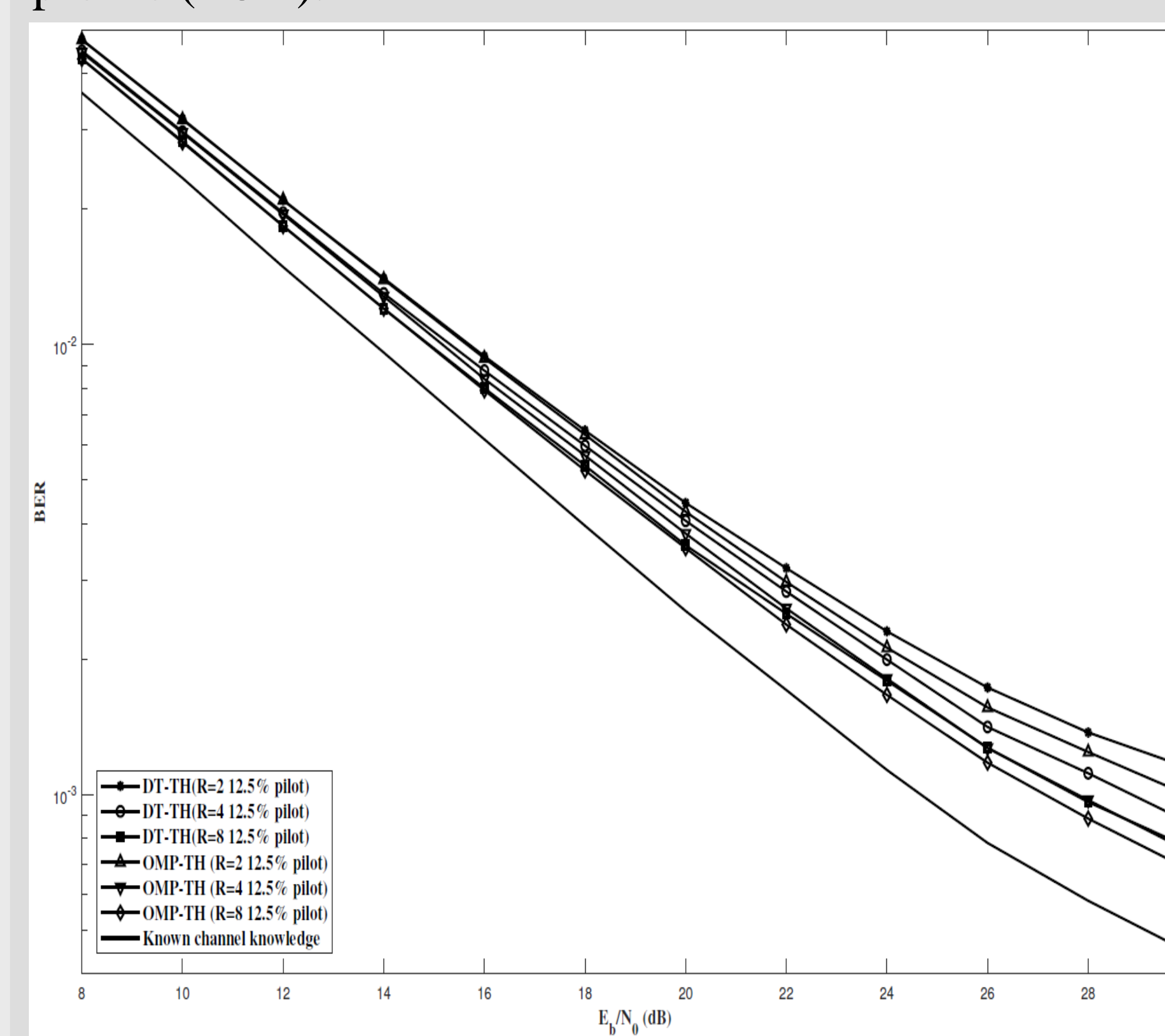
Figure 3. BER performance comparison of the proposed DT-TH method and the conventional OMP-TH method
