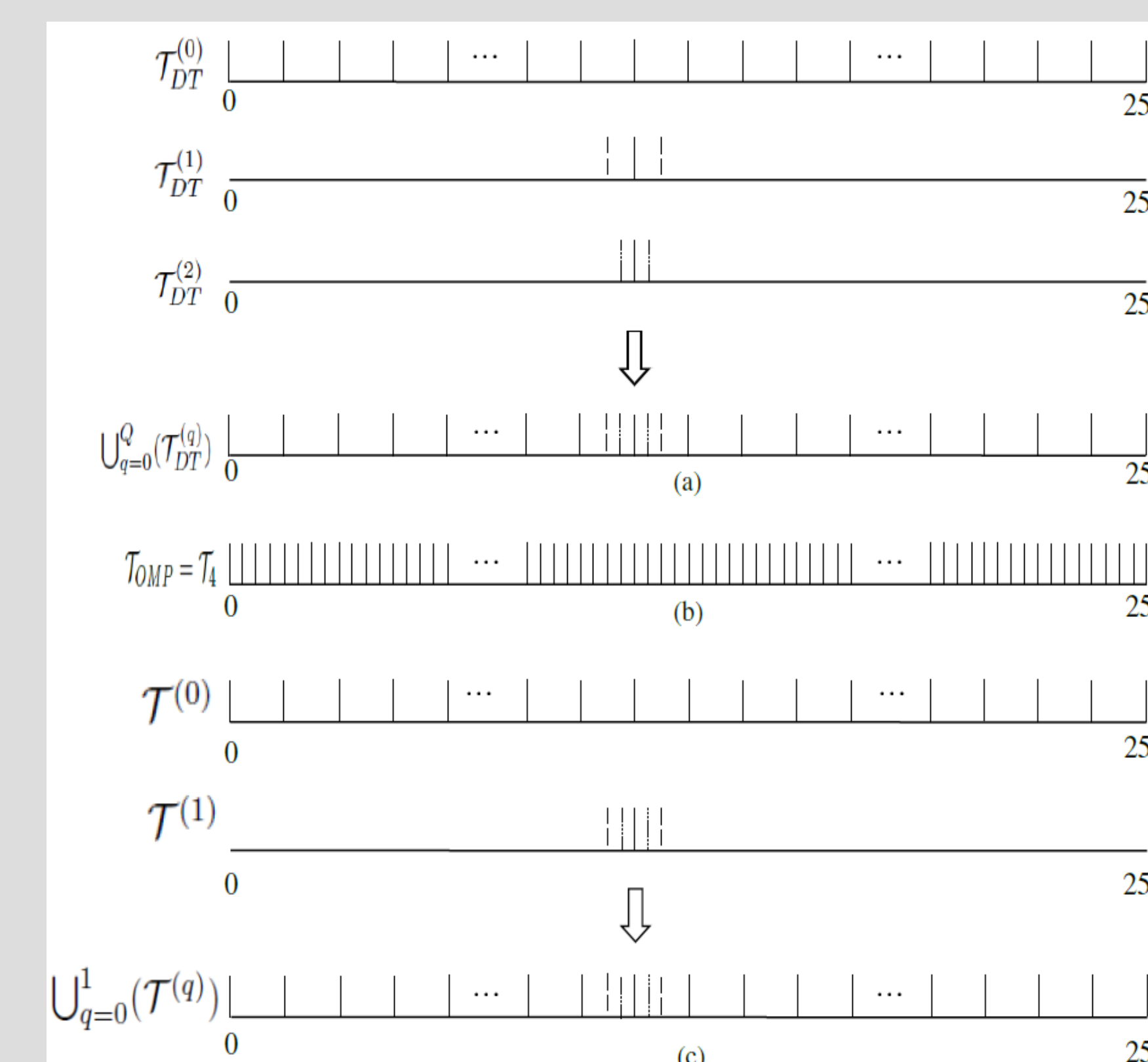
Figure 1. Tap delay grids of the method in [2] (a); tap delay grids of the OMP algorithm (b); Tap delay grids of the proposed method (c)
