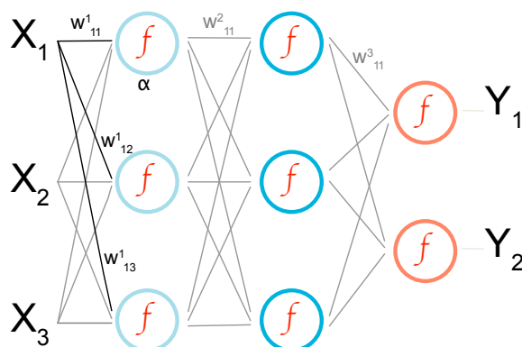
Figure 1. A representation of a neural network mapping from X_i to Y_j using three layers. Circles represent neurons using f as the activation function, and lines are adjustable weights w_{ij}^\alpha for the input values. In this case, the output of the neuron \alpha would be f(\sum_i w_{i1}^1 X_i) .
