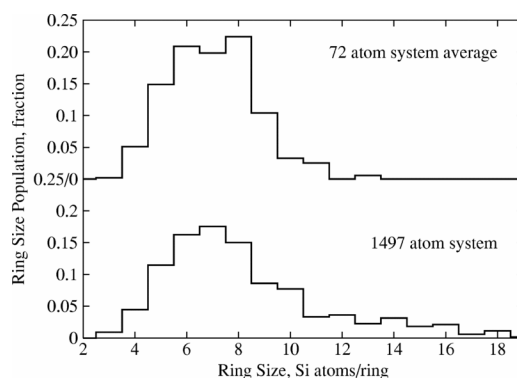
Figure 2. Ring size distribution in silica glass, as computed from 18 small (72 atoms) replicas, or a single big (1497 atoms) simulation. Reprinted with permission from Ref. 40. Copyright 2005 by the American Physical Society.
