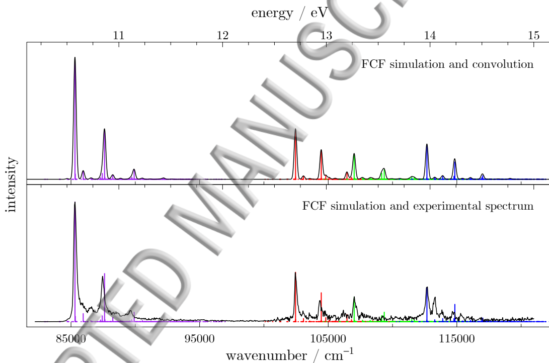
FIG. 3. Calculated photoelectron spectrum of \text{HC}_5\text{N} toward the X^+ , A^+ , B^+ , and C^+ cationic states displayed as purple, red, green, and blue stick spectra, respectively. The vibrational progression of each electronic transition has been shifted to match the experimental origin bands. See text for details.
