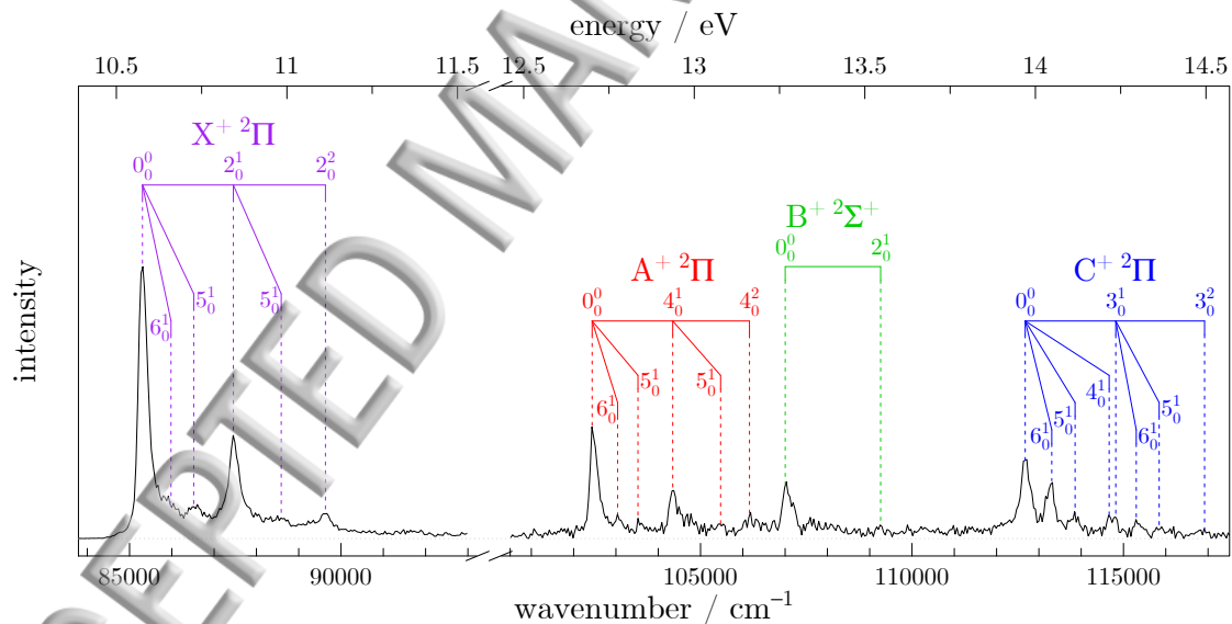
FIG. 4. TPE spectrum of HC 5 N with the vibrational band assignments according to ab initio and Franck-Condon factor calculations. The mode labelling is the same as that used in Figure 1.
