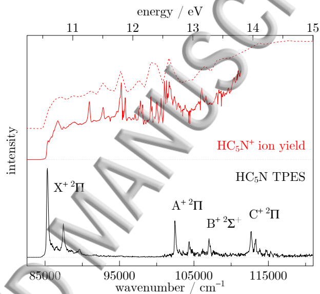
FIG. 2. \text{HC}_5\text{N}^+ ion yield (upper panel; continuous and dashed red curves) and TPE spectrum of \text{HC}_5\text{N} (lower panel; black curve) between 84\,000 and 120\,000\text{ cm}^{-1} . Depletion lines observed in the ion yield are due to absorption transitions of atomic species present in the gas filter. The red continuous line curve corresponds to a moderate extraction field that allows for detection of ions in coincidence with the photoelectron with 3.7\text{ eV} maximum kinetic energy. The red dashed ion yield displays the same signal but with a higher extraction field and a lower spectral resolution, in order to cover the full range up to 120\,000\text{ cm}^{-1} .
