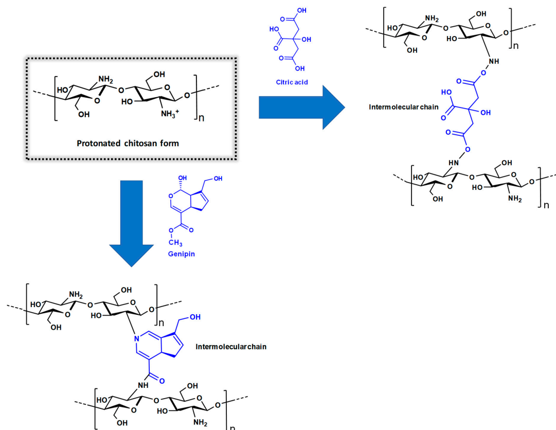
Figure 5. The mains cross-linking reactions using chitosan.
