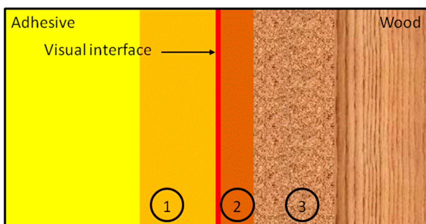
Figure 10. Schematic representation of the interfacial zone between adhesive and wood. 1: adhesive boundary layer, 2: interface between boundary layer and wood substrate which constitutes the adhesion mechanism (mechanical interlocking, covalent bonding, or secondary chemical bonds), and 3: adhesive penetration zone.
