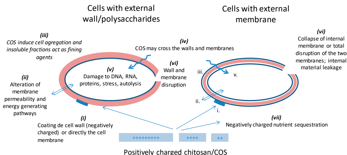
Figure 6. Inventory of the different molecular processes that may contribute to the chitosan antimicrobial activity (adapted from [79]). The numbers (i) to (vii) correspond to those used in the text (see above).
