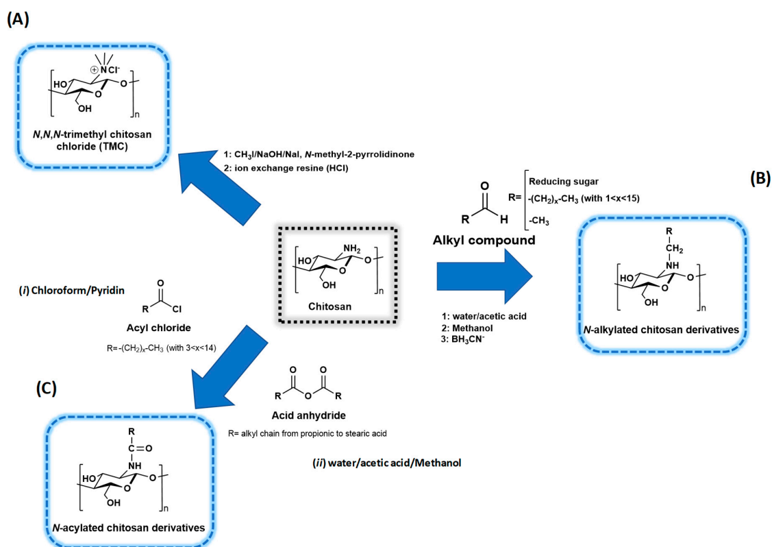
Figure 3. Production of chitosan derivatives by different methods: (A) Quaternization, (B) N-alkylation, and (C) N-acylation.
