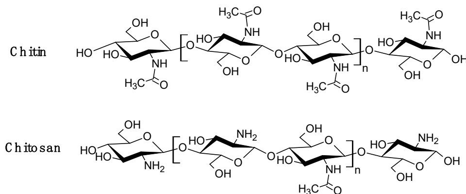
Figure 1. Chemical structure of chitin and chitosan.
