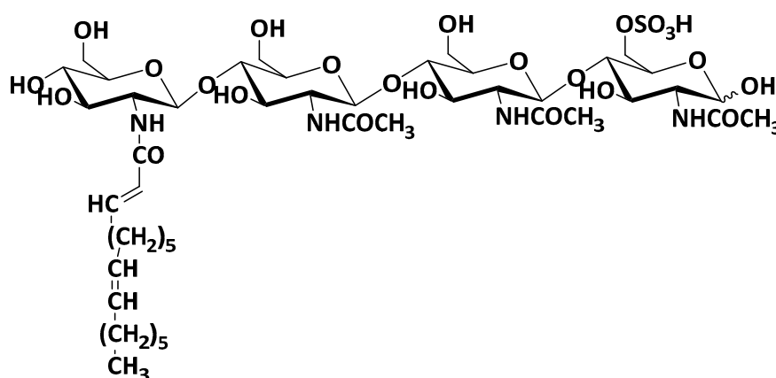
Figure 8. Structure of lipo-chitoooligosaccharides produced by EJ355 strain from S. meliloti [159].
