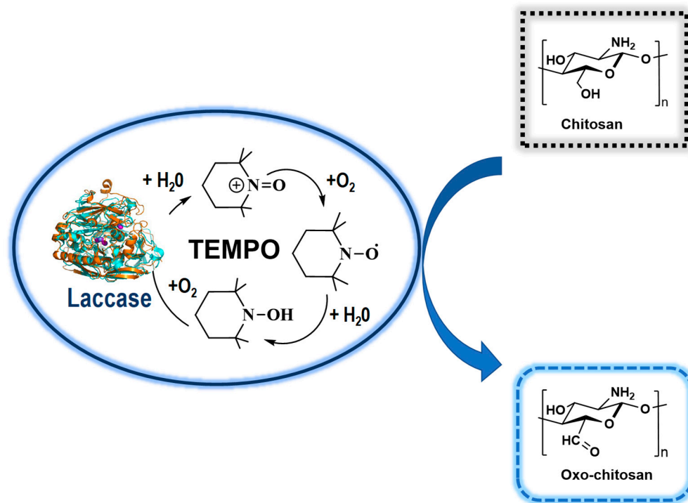
Figure 4. Environmentally friendly oxidation of CS via TEMPO/laccase system (adapted from [52]).
