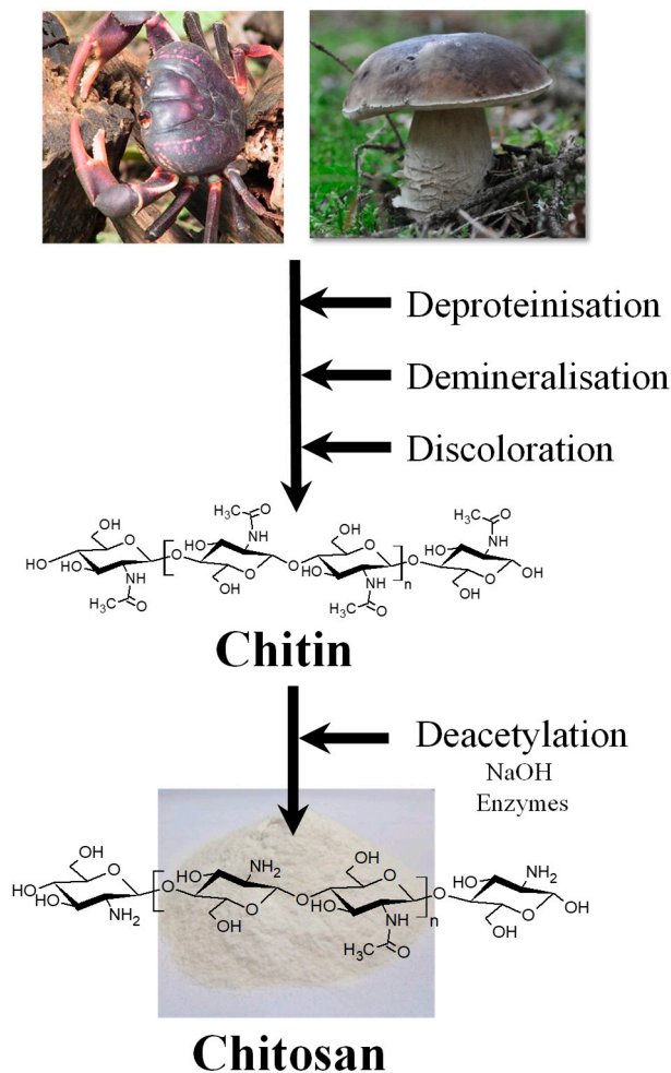
Figure 2. General steps for chitin and chitosan production.
