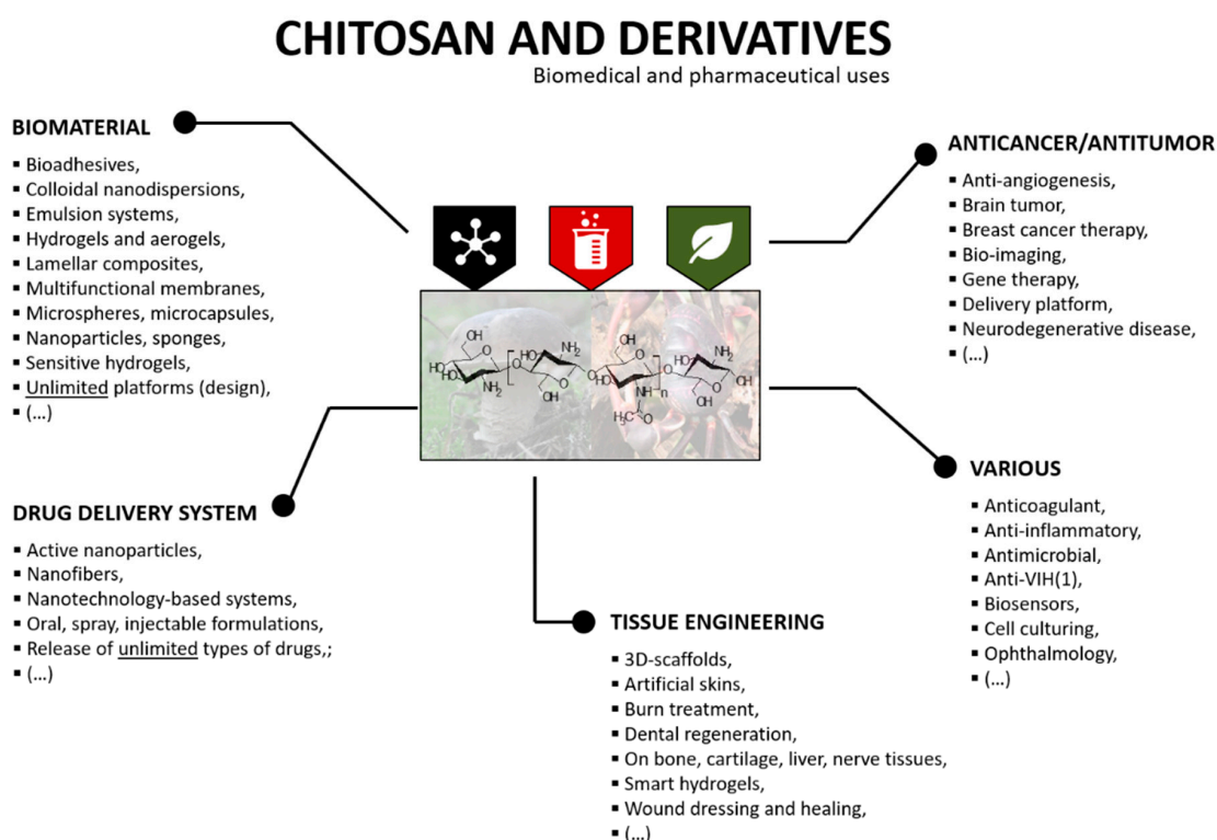
Figure 9. Various applications of chitosan and derivatives in biomedical and pharmaceutical fields.
