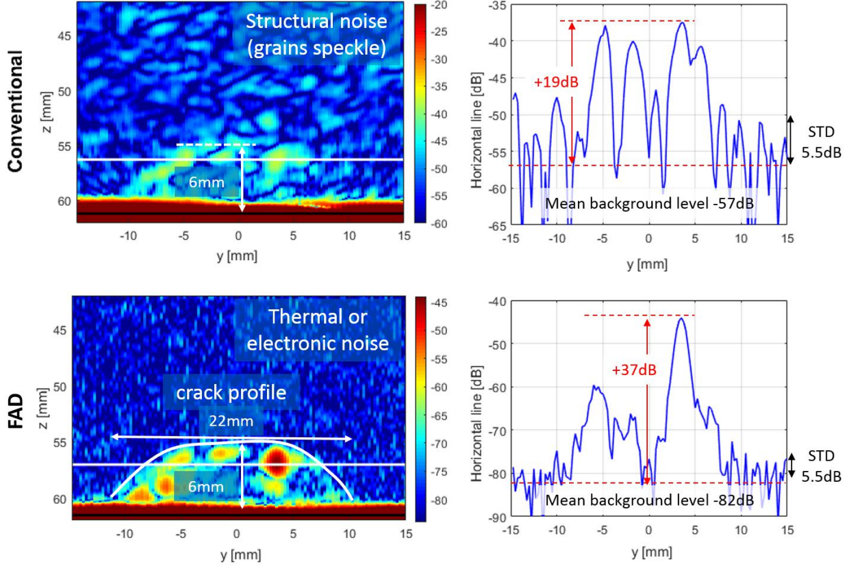
Fig. 4. [Thermal fatigue crack specimen] Contrast and background noise comparison between the conventional (i.e. linear) and the fundamenta wavel amplitude difference (FAD) (i.e. nonlinear) methods performed with electronic beam steering along the crack direction (i.e. parallel scan)
