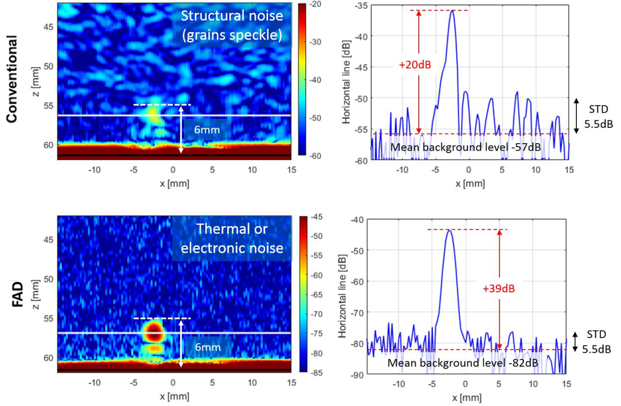
Fig. 3. [Thermal fatigue crack specimen] Contrast and background noise comparison between the conventional (i.e. linear) and the fundamental wave amplitude difference (FAD) (i.e. nonlinear) methods performed with electronic beam steering across the crack direction (i.e. perpendicular scan).
