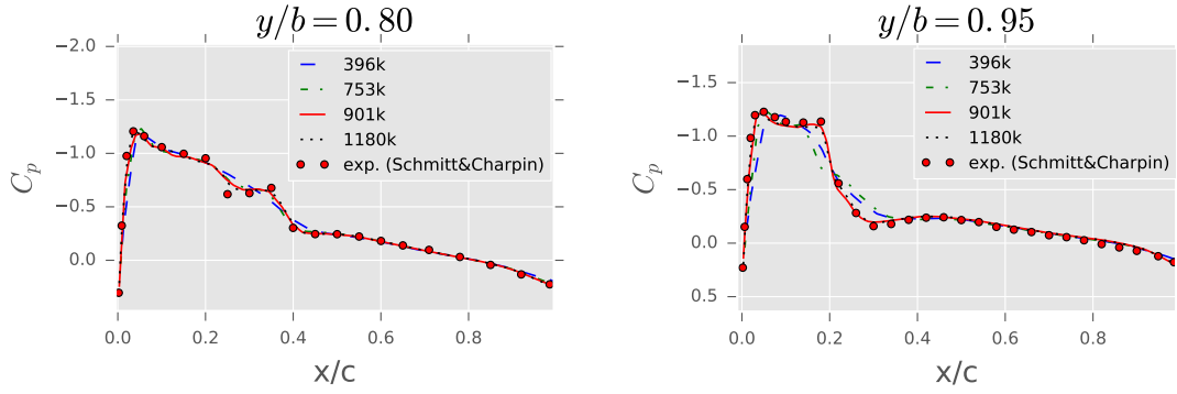
(a) The C_p distributions at z/b = 0.8 .
