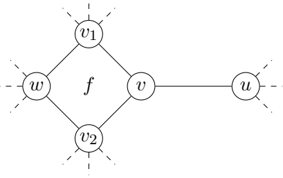
Figure 2: Reducible configuration in case (ii).
