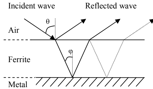
Fig.7. Ferrite tile reflectivity principle.
