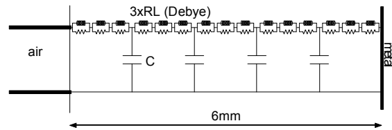
Fig.8. Equivalent 1-D TLM electric circuit for electromagnetic modelling of ferrite tiles.
