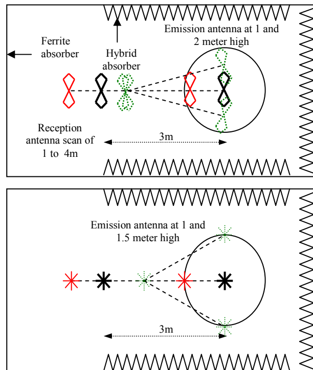
Fig.2. NSA measurements in the quiet zone of a semi-anechoic chamber for horizontal and vertical polarizations.
