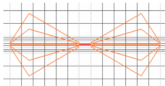
Fig.11. Meshing of the biconical antennas
