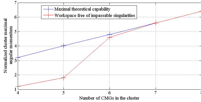
Fig. 2: Workspace free of elliptic singularity compared to the maximal capabilities
