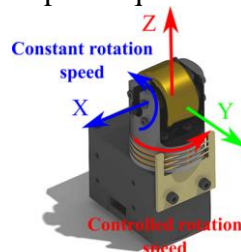
Fig.1: CMG principle
