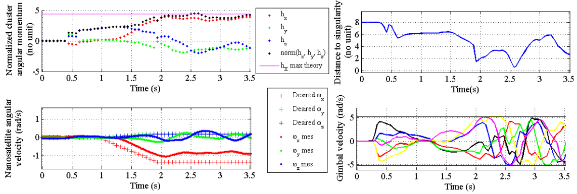
Fig. 3: Experimental results of a X-axis manoeuvre, without the varying covariance, from a favourable initial position
