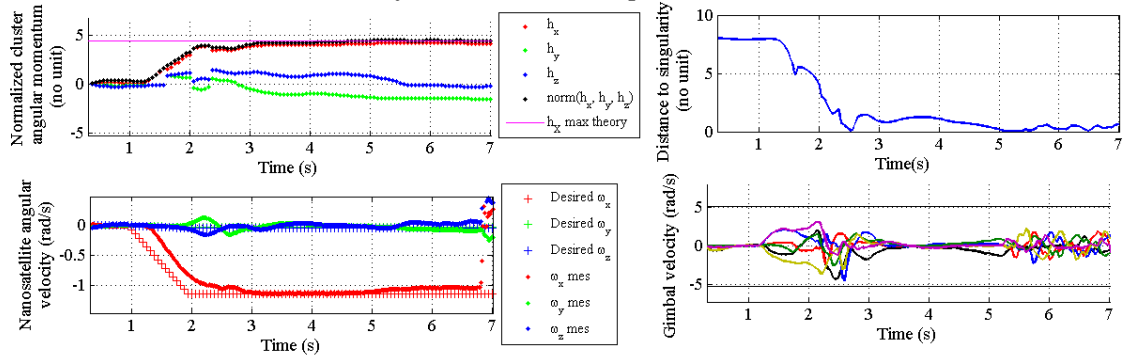
Fig. 3: Experimental results of a X-axis manoeuvre, with the varying covariance, from a favourable initial position
