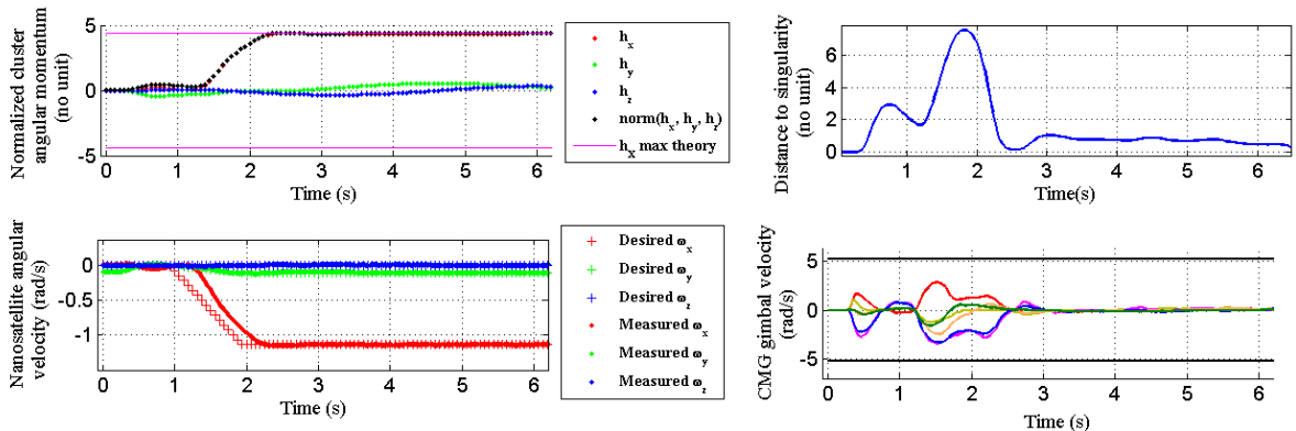
Fig. 5: Experimental results of a X-axis maneuver, with the varying covariance, from a singular initial position
