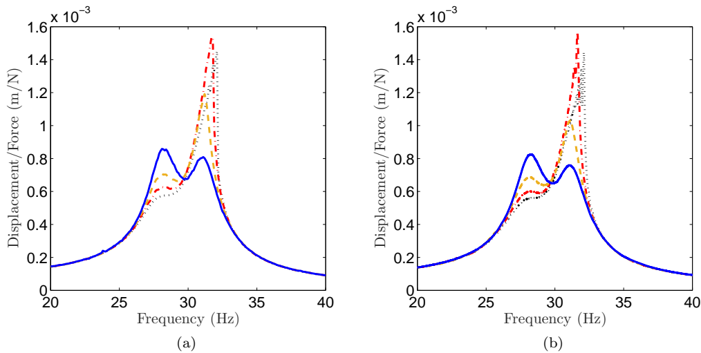
Figure 9: Frequency response functions for various forcing amplitudes with a linear resonant shunt, F = 0.2 N ( - ), F = 0.4 N ( - - ), F = 0.6 N ( - \cdot - ) and F = 0.8 N ( \cdots ) – (a) experiments, (b) simulations.
