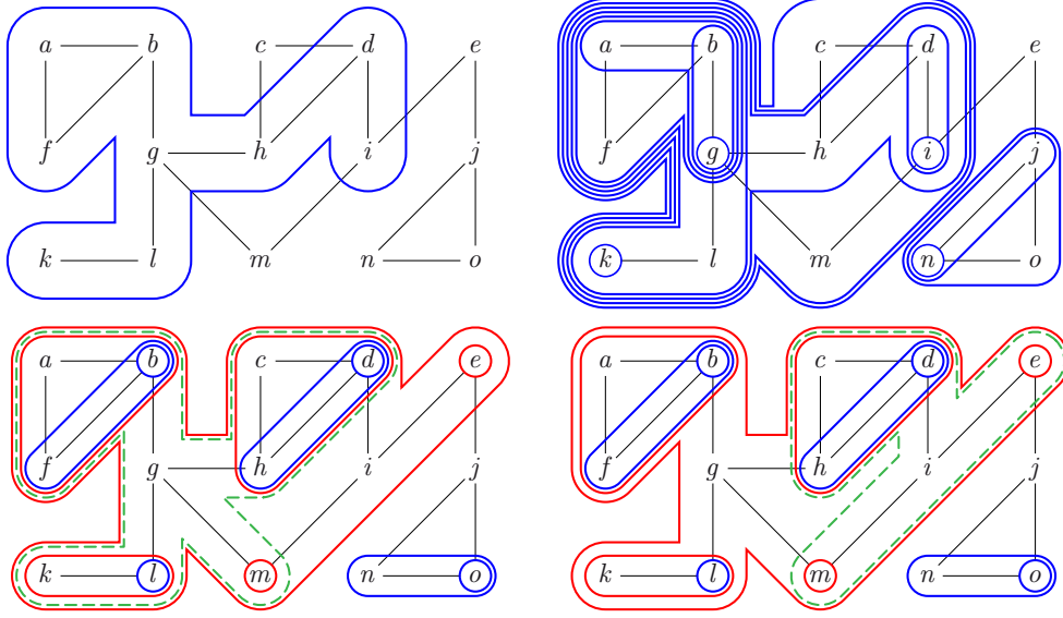
Fig. 3: A tube t_{\text{ex}}^o = \{a, b, d, f, g, h, i, k, l\} of G_{\text{ex}} (top-left), a maximal tubing T_{\text{ex}}^o on G_{\text{ex}} (top-right) and two maximal tubings related by a flip (bottom): the two exchanged tubes t_{\text{ex}} = \{a, b, c, d, f, g, h, k, l, m\} and t'_{\text{ex}} = \{c, d, e, h, i, m\} are in dotted green while the six forced tubes are in red, and the seven others are in blue.
