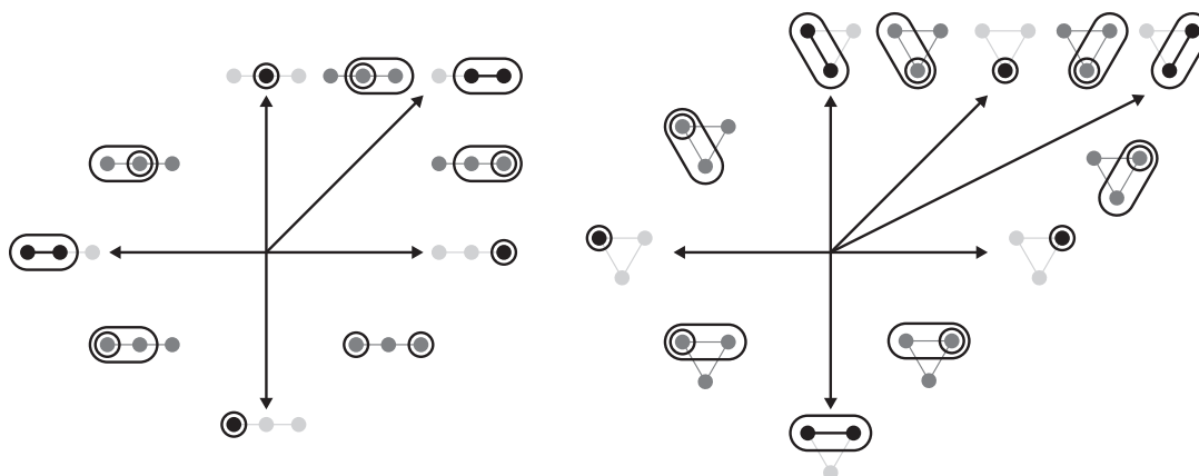
Fig. 4: Compatibility fans of the 3-path (left) and of the triangle (right).
