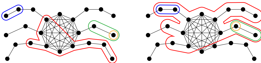
Fig. 9: A spider with a tubing T (left) and its image \Omega(T) (right) by the nested complex automorphism \Omega of the spider.
