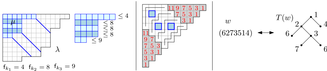
Fig. 2: Left: Given a skew shape \lambda/\mu , for each corner k of \mu we record the last row f_k of \lambda from diagonal d_{\mu_k - k} . These row numbers give the bound for the flagged tableaux of shape \mu . Center: the hook-lengths of an excited diagram of \delta_{3+8}/\delta_3 corresponding to the 4-fan of Dyck paths on the right. Right: The full binary tree corresponding to the alternating permutation w = (6273514) .
