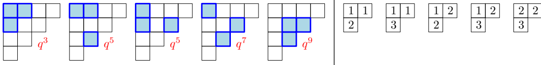
Fig. 1: Left: the C_3 = 5 excited diagrams for (4321/21) , their associated statistic a(D) , right: the five corresponding flagged tableaux in \mathcal{F}(\mu, (2, 3)) .
